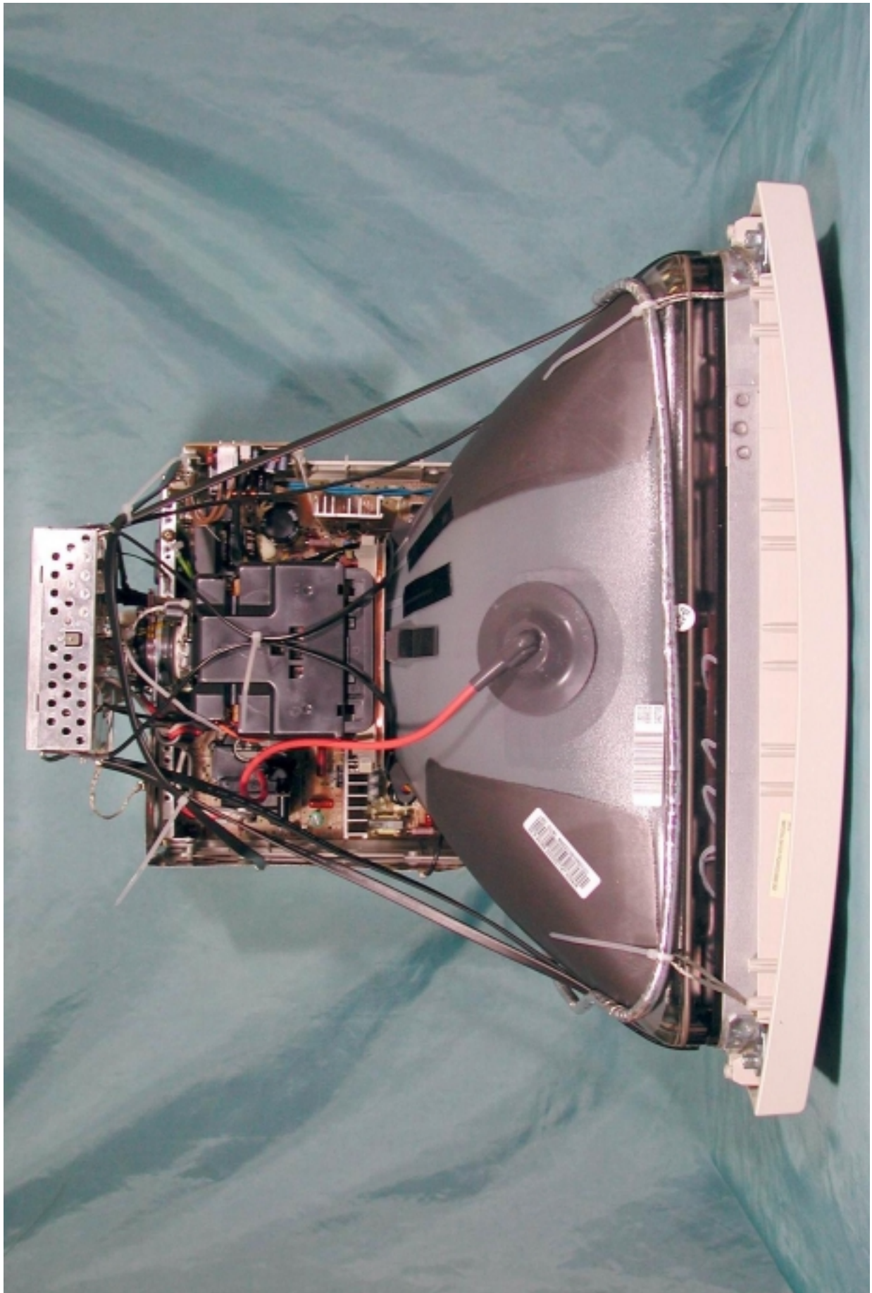
Top View Without Back Cover
