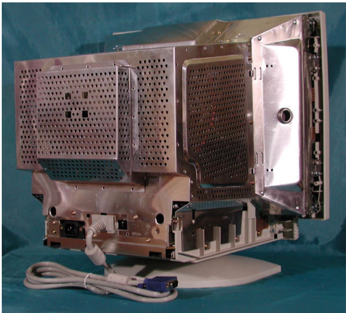
Side View w/o Back Cover
