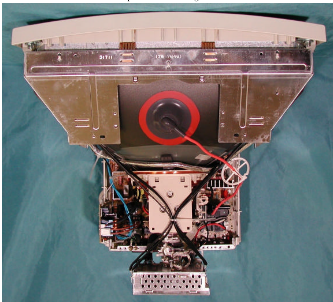
Top View w/o Shielding Cover
