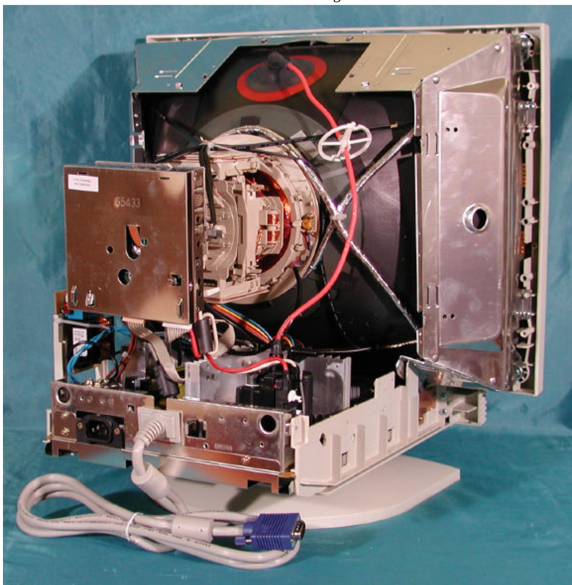
Side View w/o Shielding Cover
