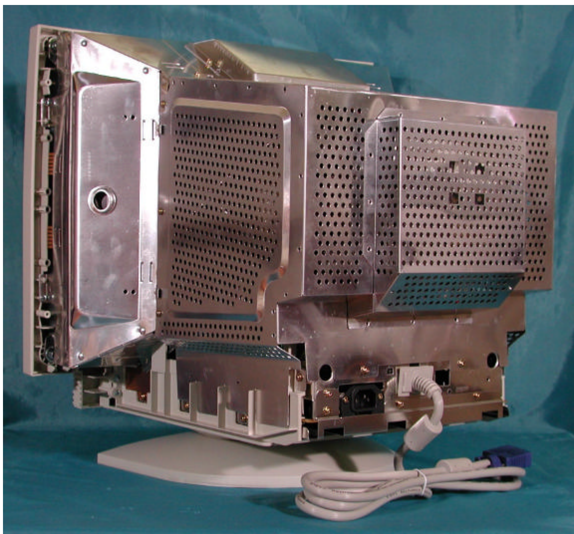
Side View w/o Back Cover
