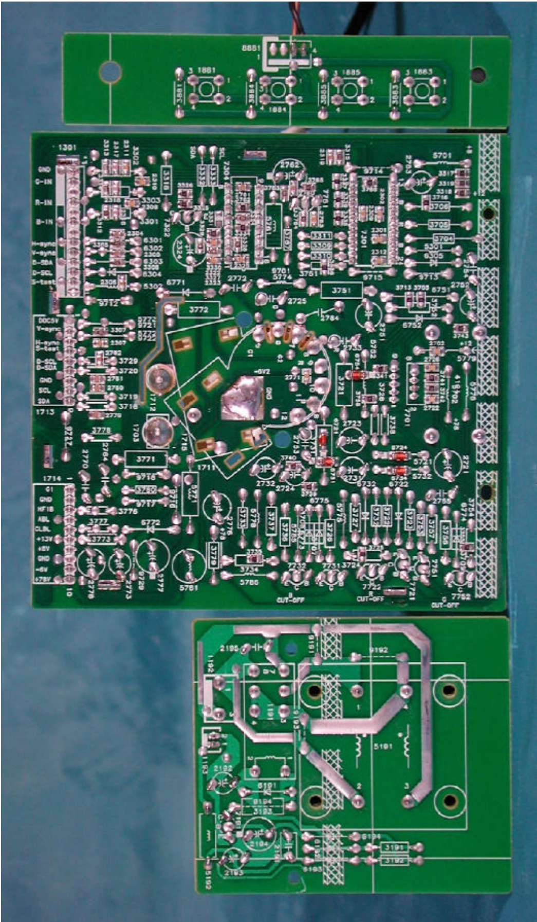
PCB Layout
