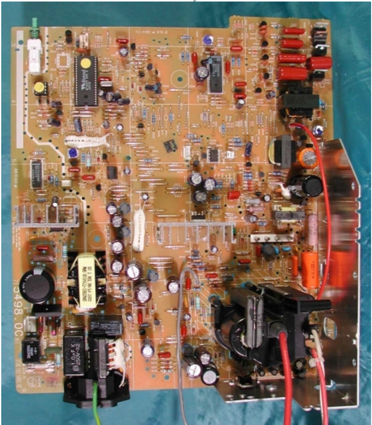
PCB Layout
