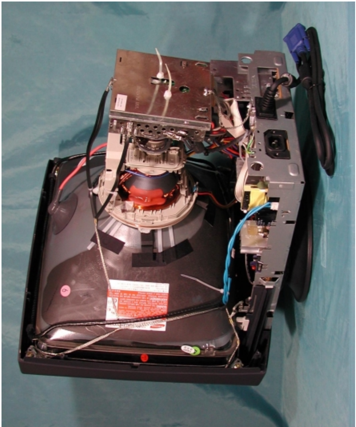
Side View
