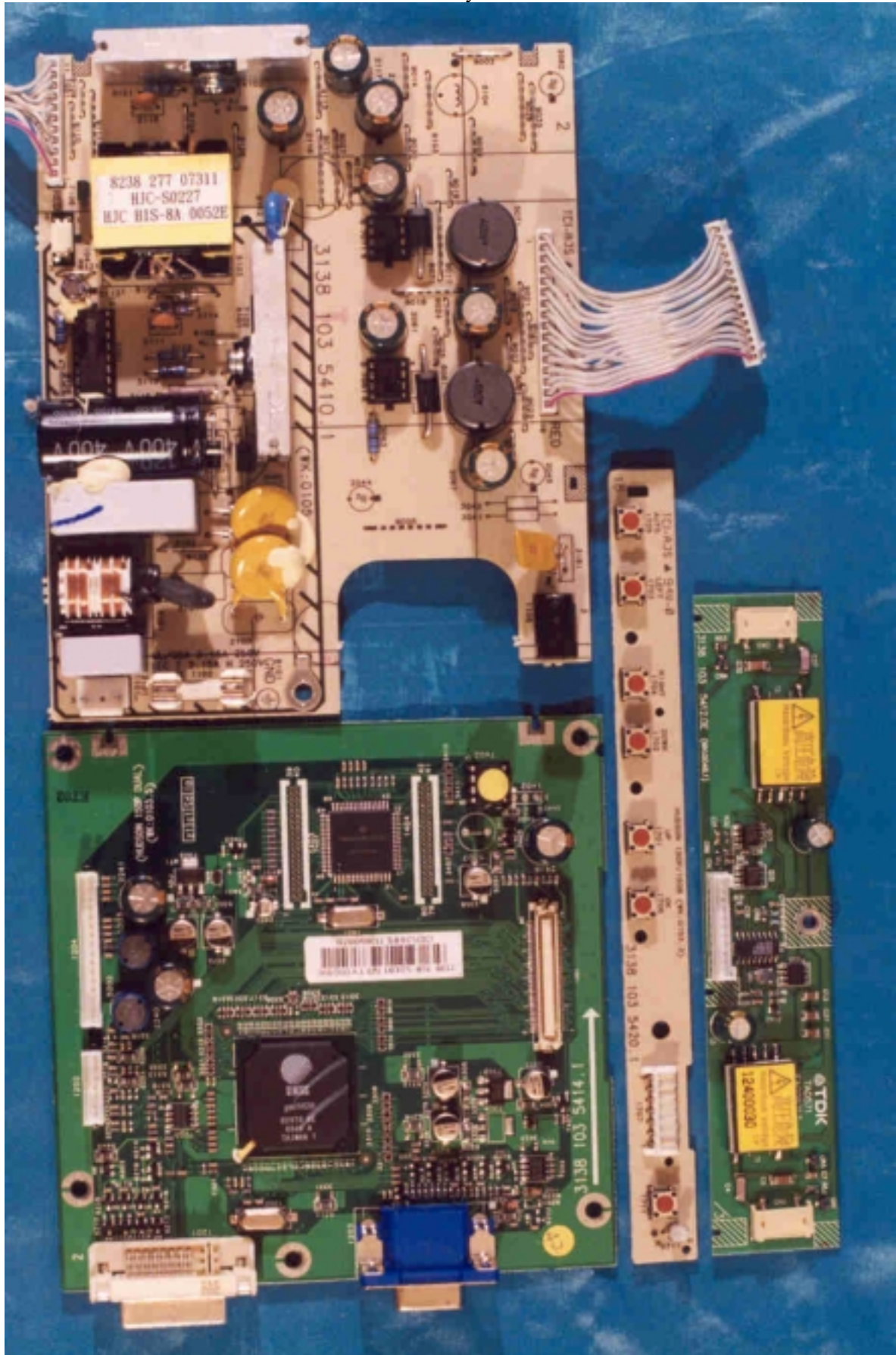
PCB Layout
