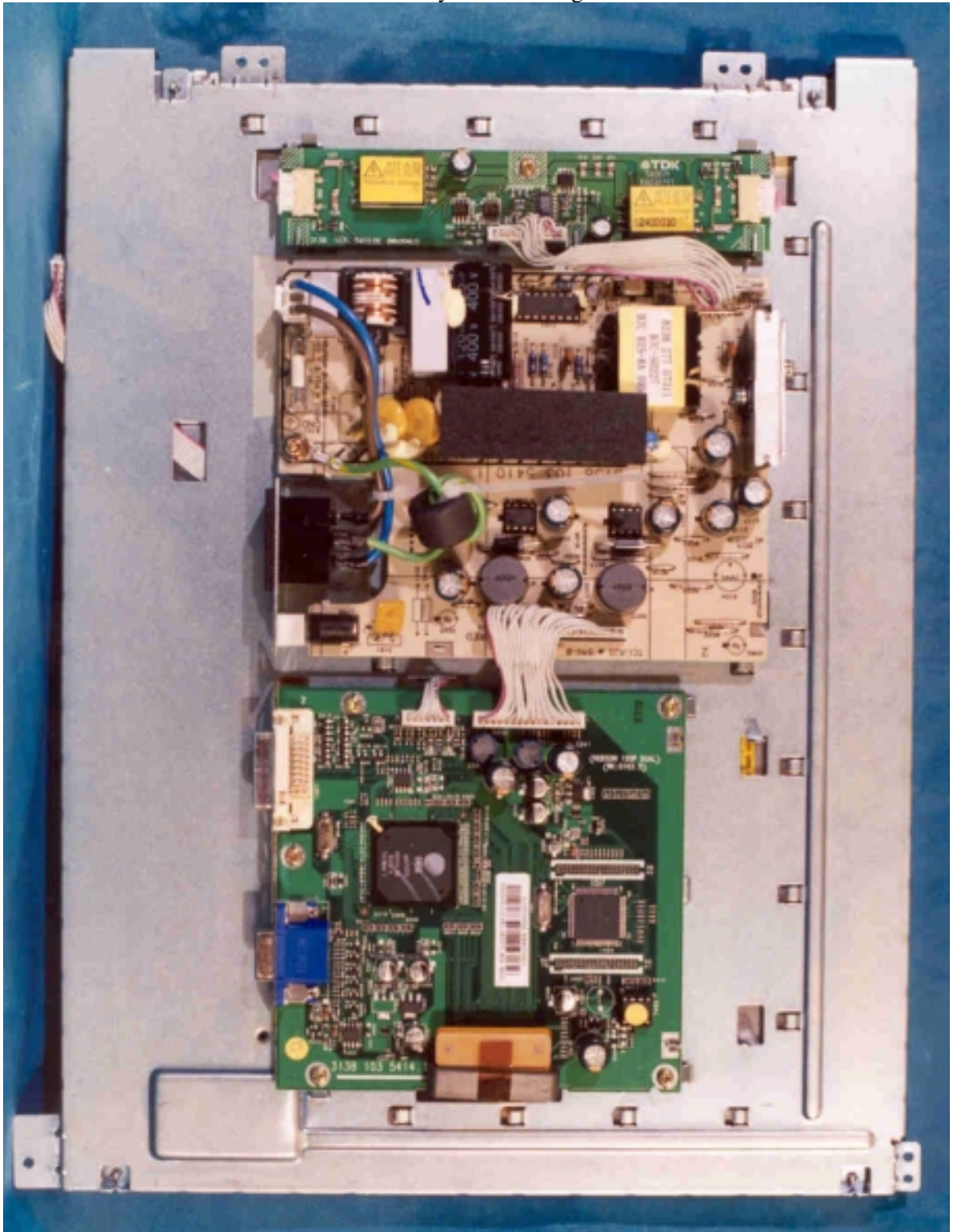
LCD Assembly w/o Shielding Cover
