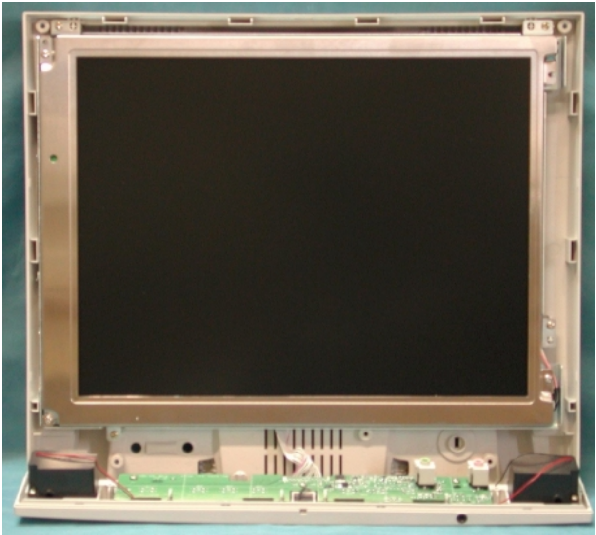
Front View w/o Front Cabinet
