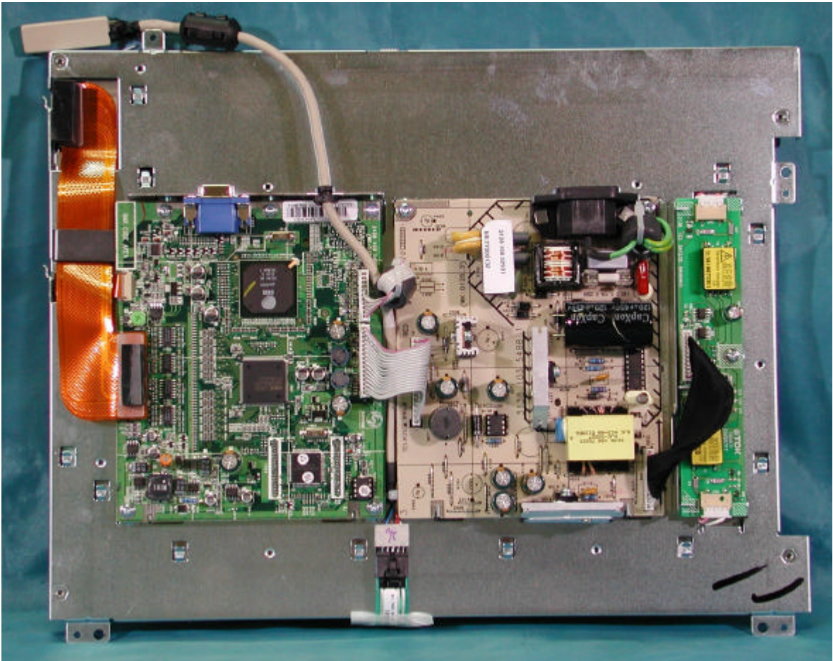
Panel Assembly w/o Shielding Cover
