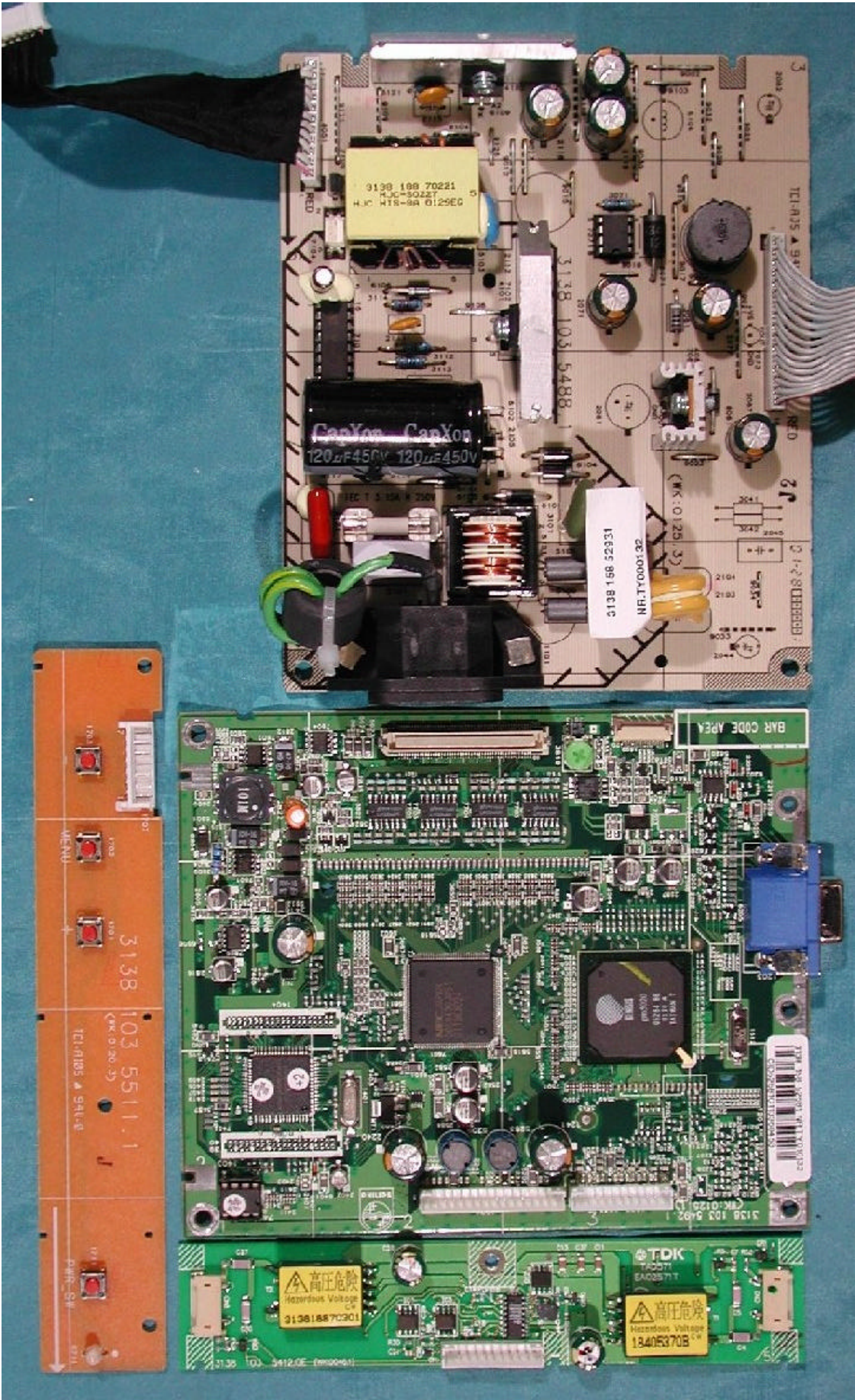
PCB Layout
