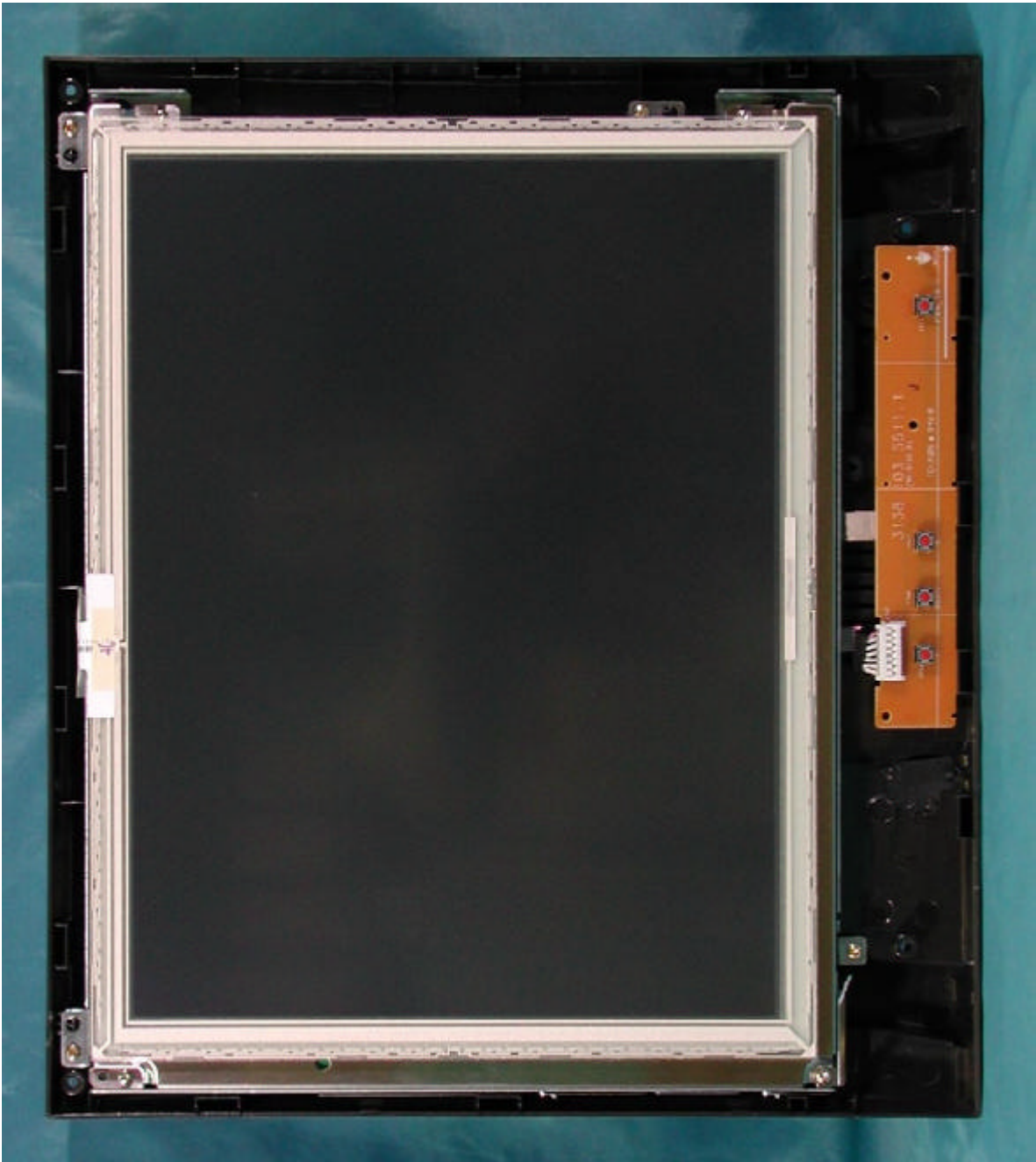
Front View w/o Front Cabinet
