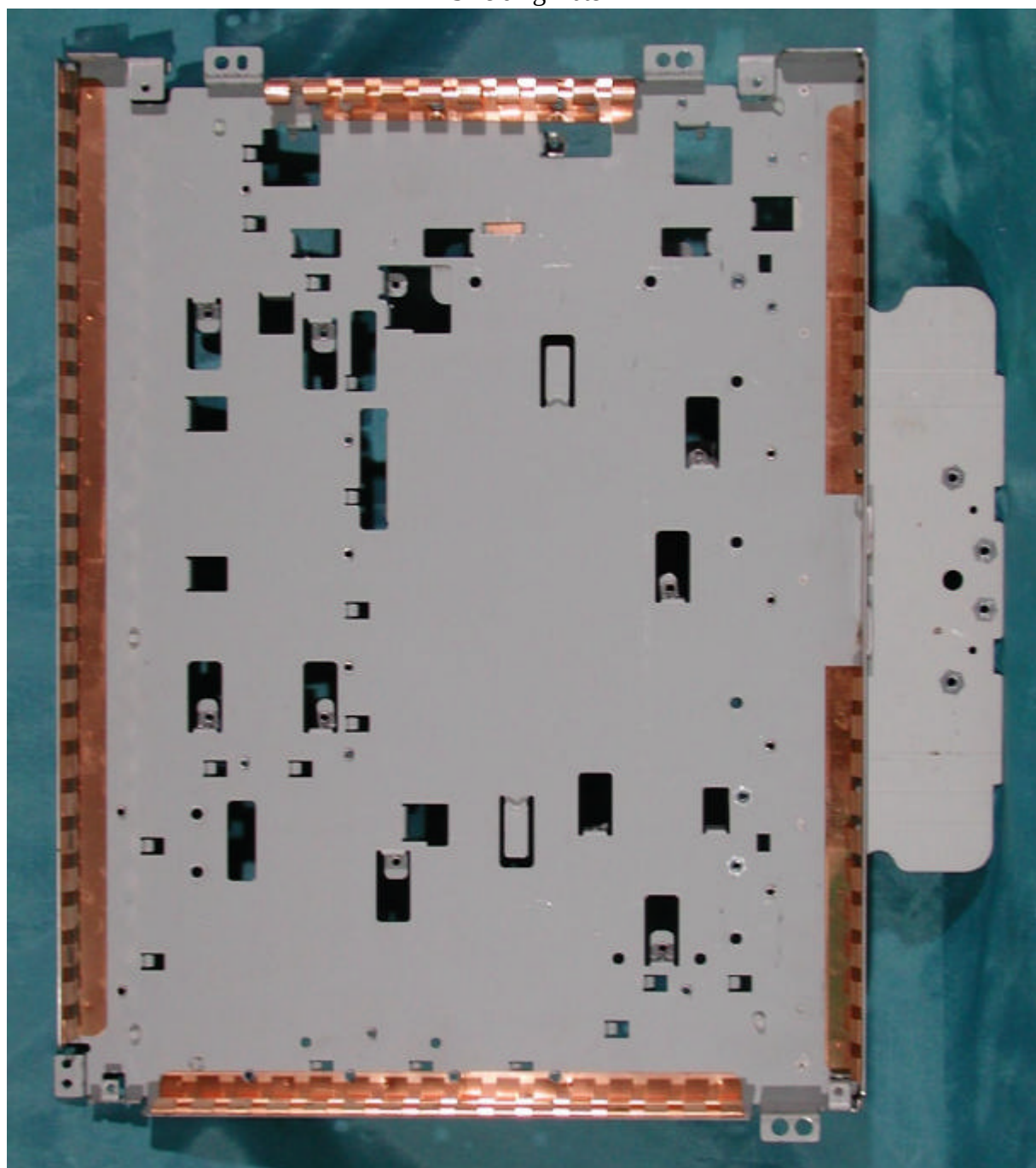
Shielding Plate
