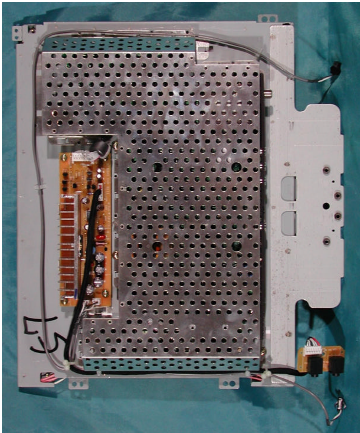
Rear View w/o Cabinets
