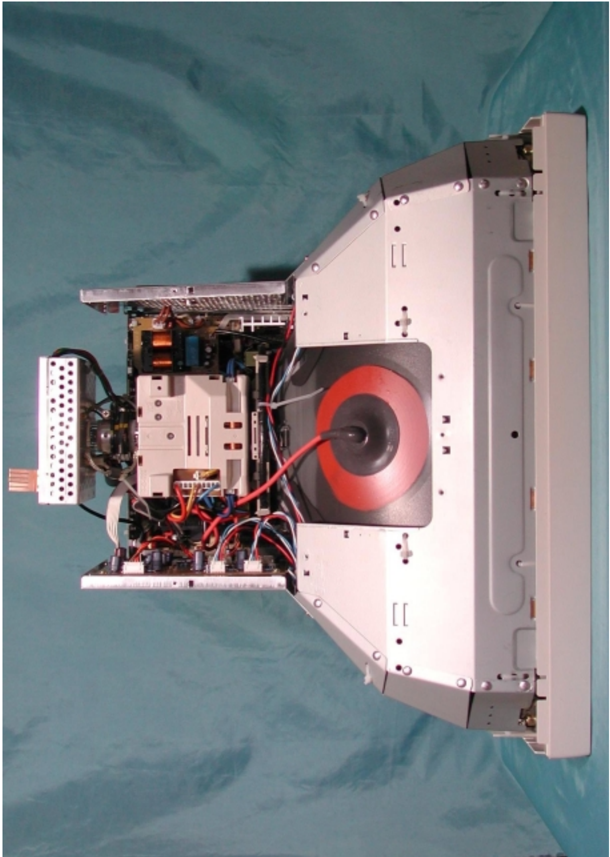
Top View Without Shielding Cover
