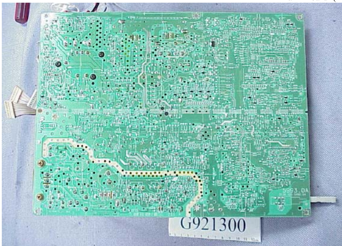
Figure 20 Display Color Monitor Main Board (Foil Side)
