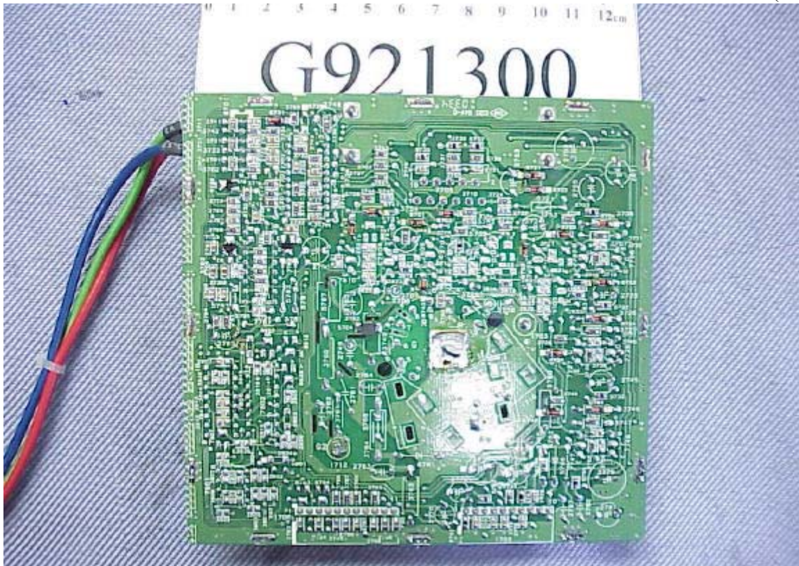
Figure 18 Display Color Monitor Video Board (Foil Side)
