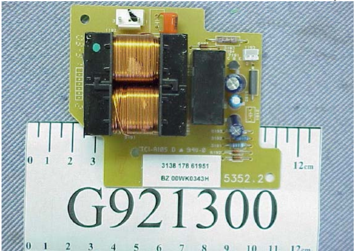
Figure 21 Display Color Monitor Transformer Board (Component Side)
