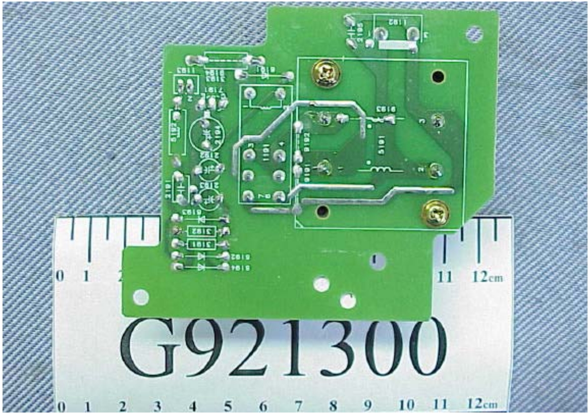
Figure 22 Display Color Monitor Transformer Board (Foil Side)
