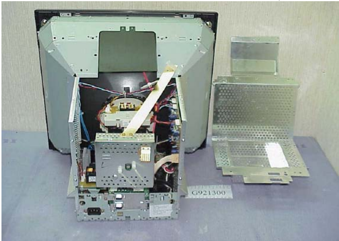
Figure 8 Display Color Monitor Internal View (Remove Drive Board & Side Shield Covers)
