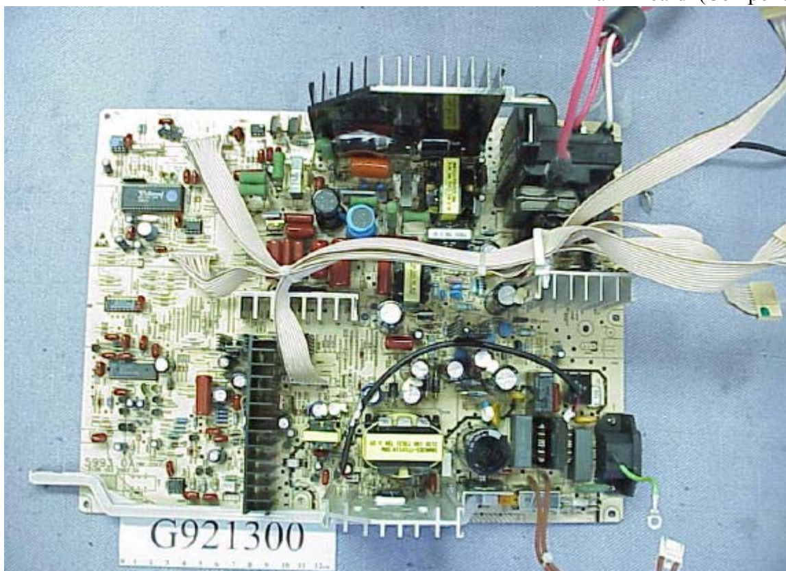
Figure 19 Display Color Monitor Main Board (Component Side)
