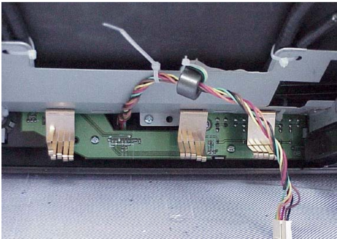
Figure 25 Display Color Monitor Internal View
