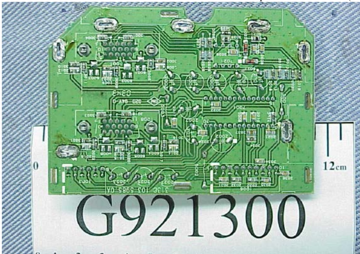
Figure 24 Display Color Monitor Input Interface Board (Foil Side)
