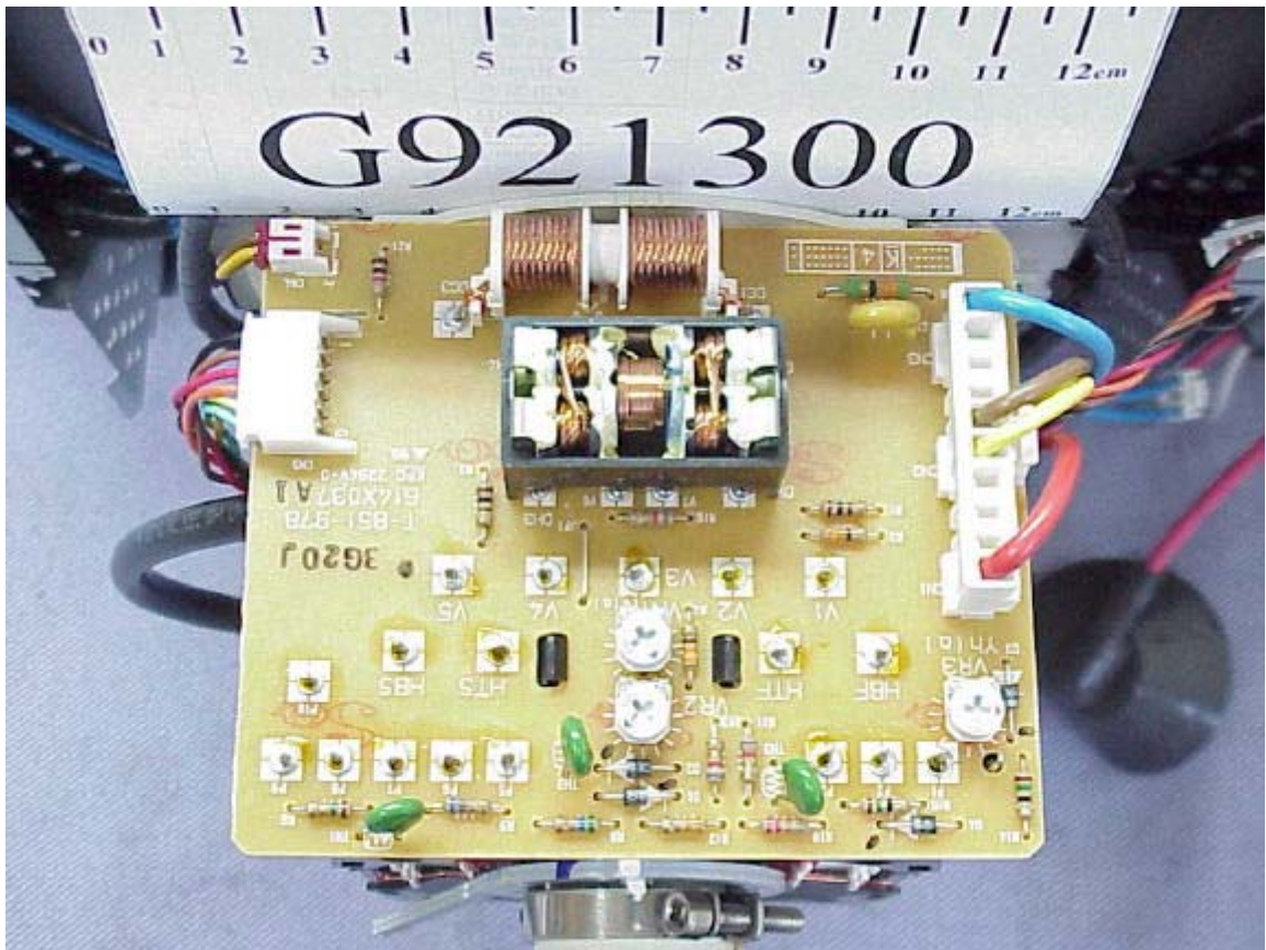
Figure 12 Display Color Monitor Deflection Board
