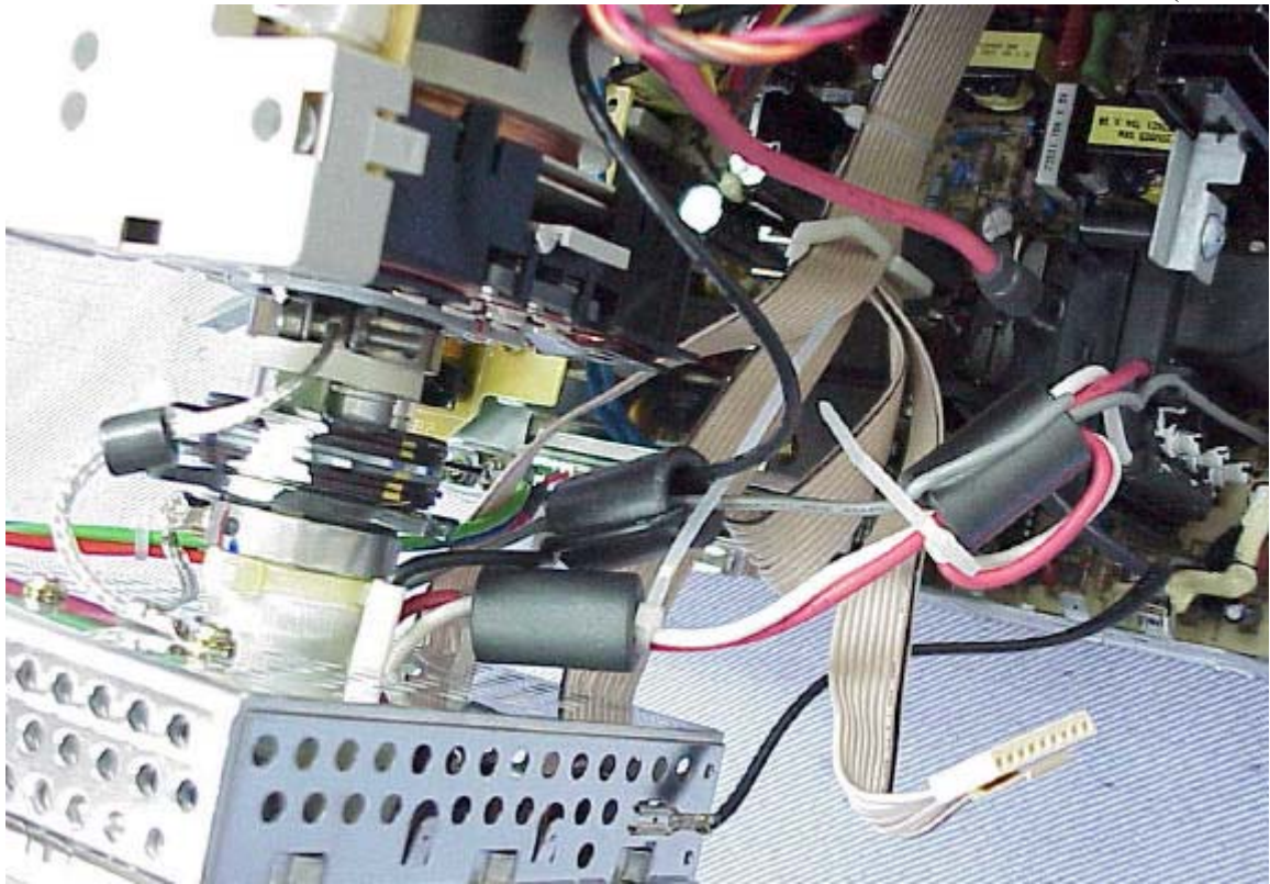
Figure 10 Display Color Monitor Internal View (Remove Video Board)
