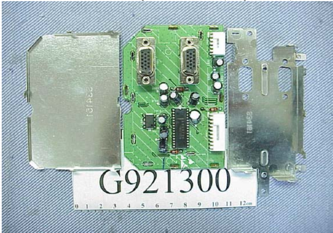
Figure 23 Display Color Monitor Input Interface Board (Component Side) & Shield Covers
