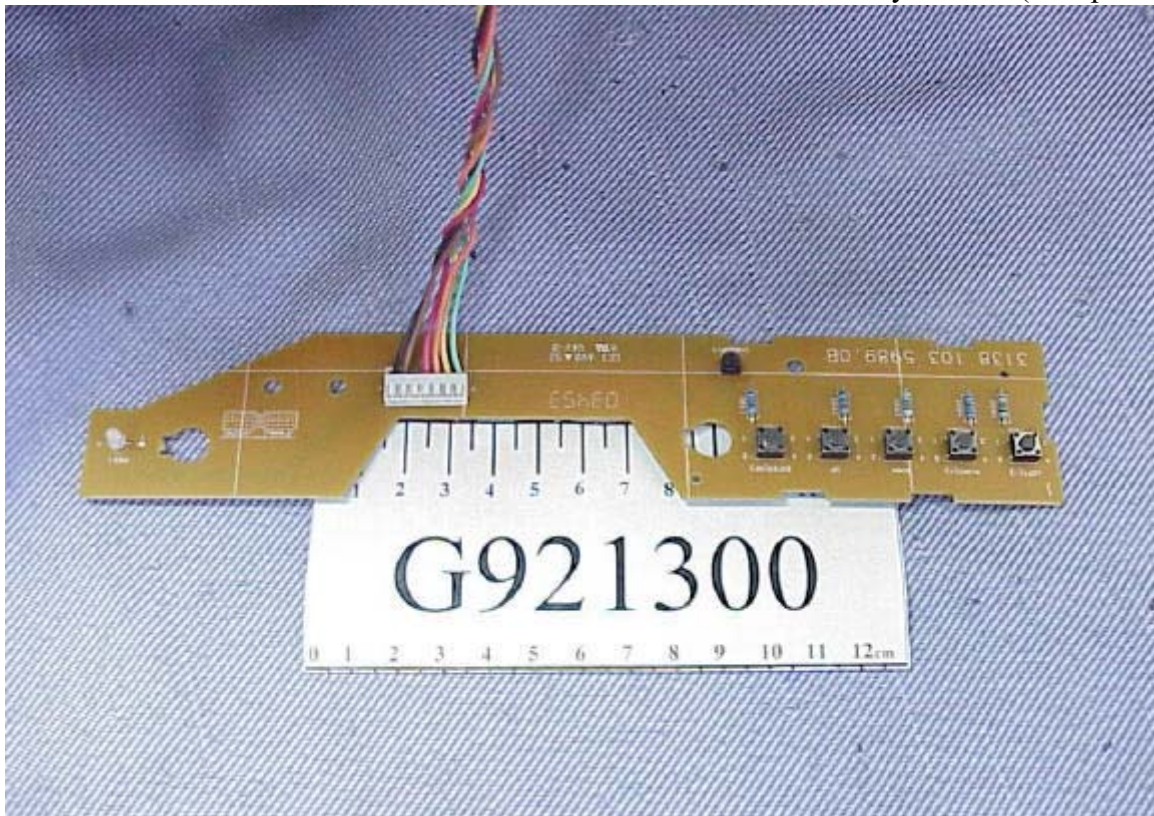
Figure 26 Display Color Monitor Function Key Board (Component Side)
