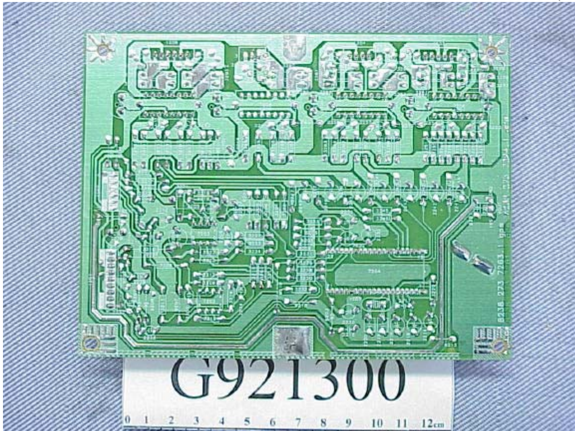
Figure 15 Display Color Monitor Drive Board (Foil Side)
