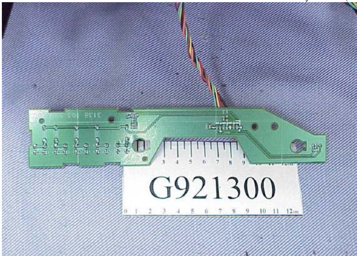
Figure 27 Display Color Monitor Function Key Board (Foil Side)
