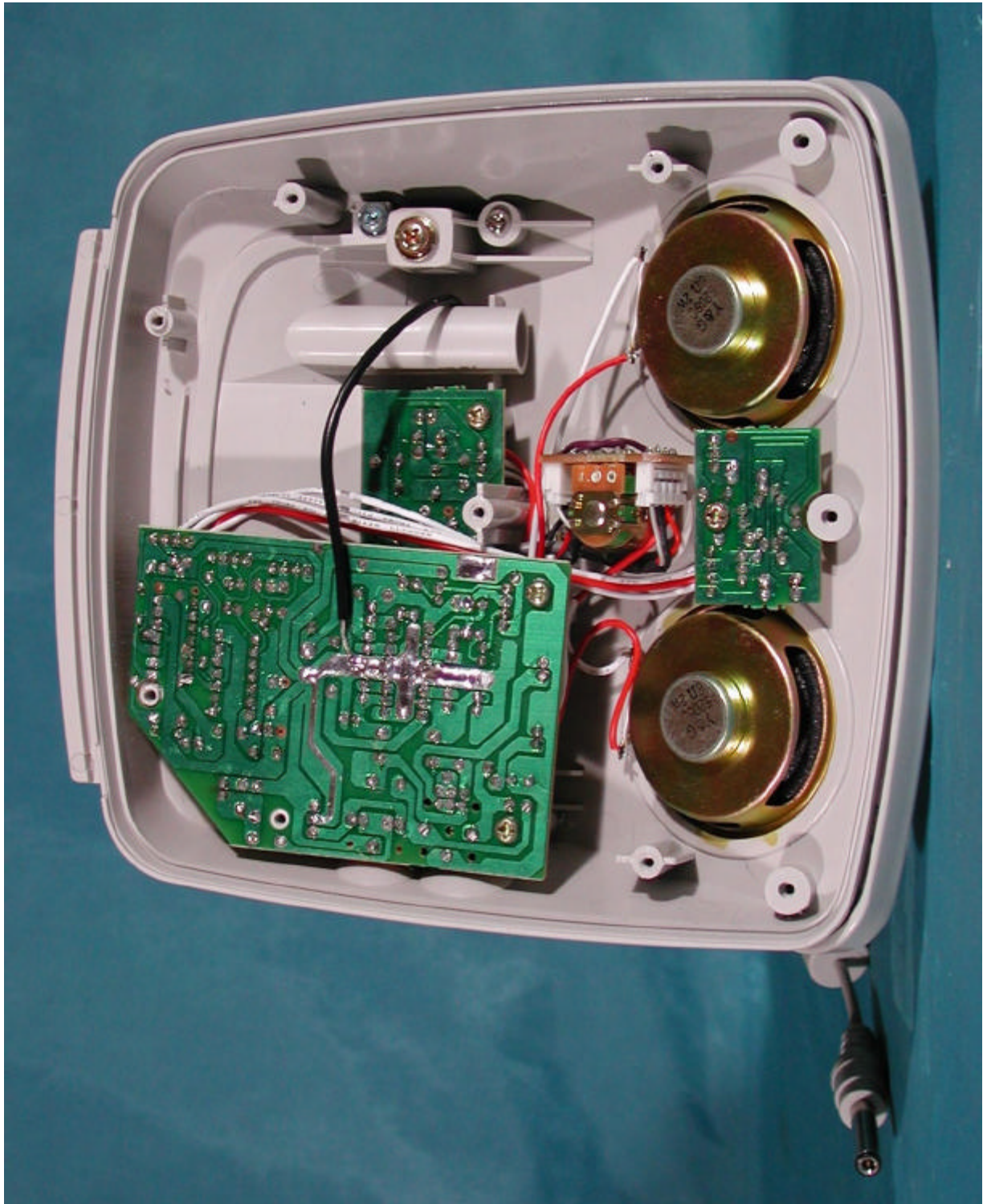
Audio Assembly
