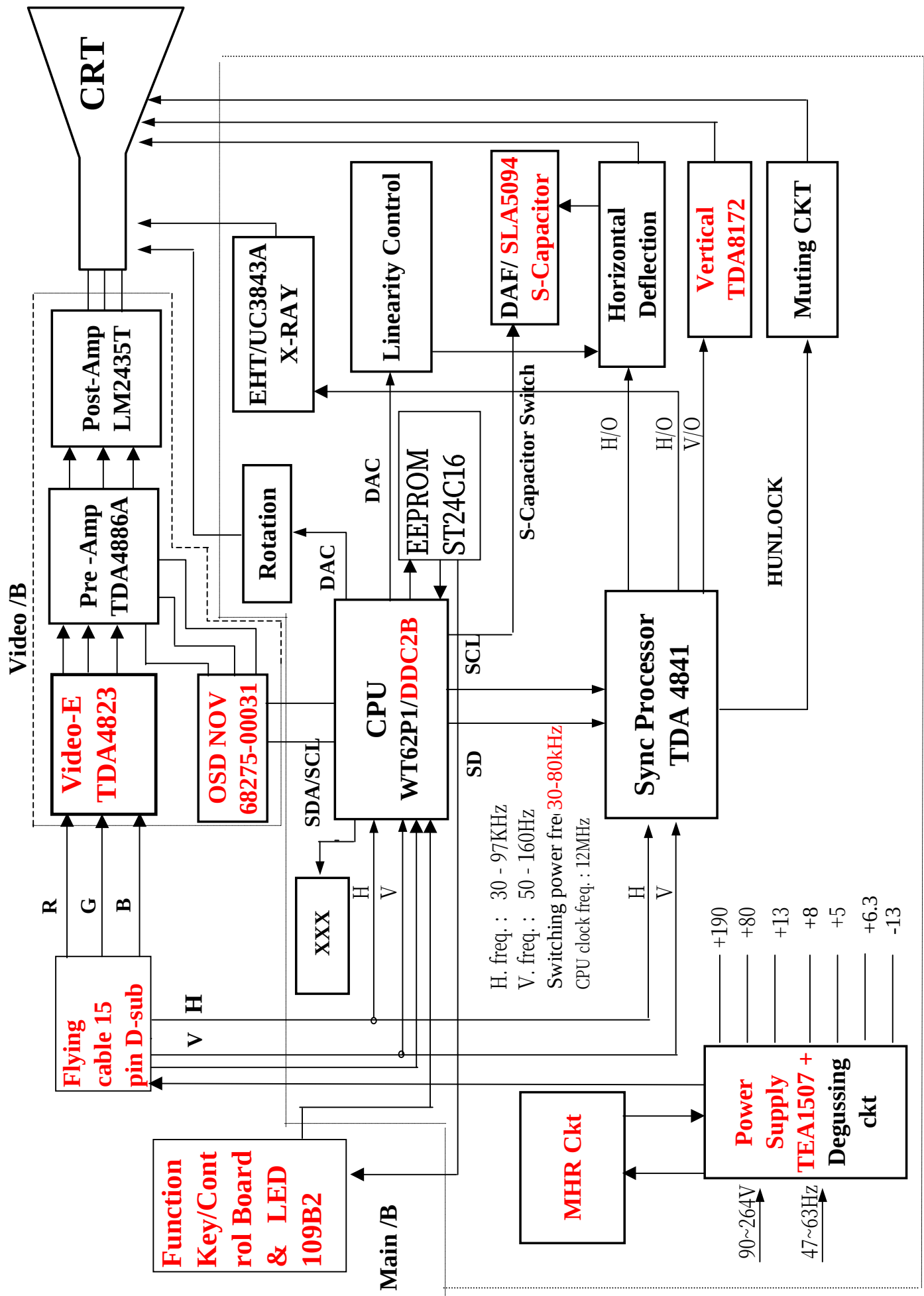
107P4 17" 92KHz BUS-DRIVER MONITOR
