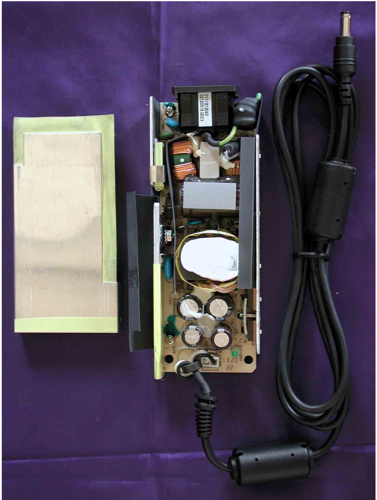
Adapter Assembly w/o Shielding
