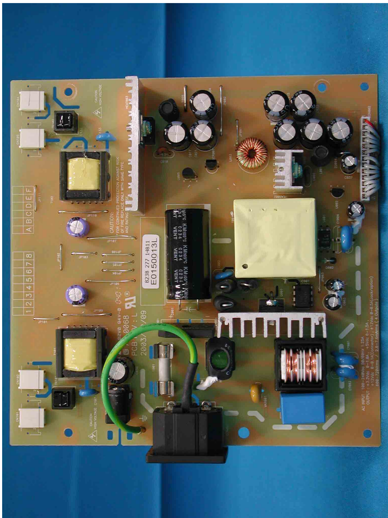
PCB Layout (Lien-Channg Power)
