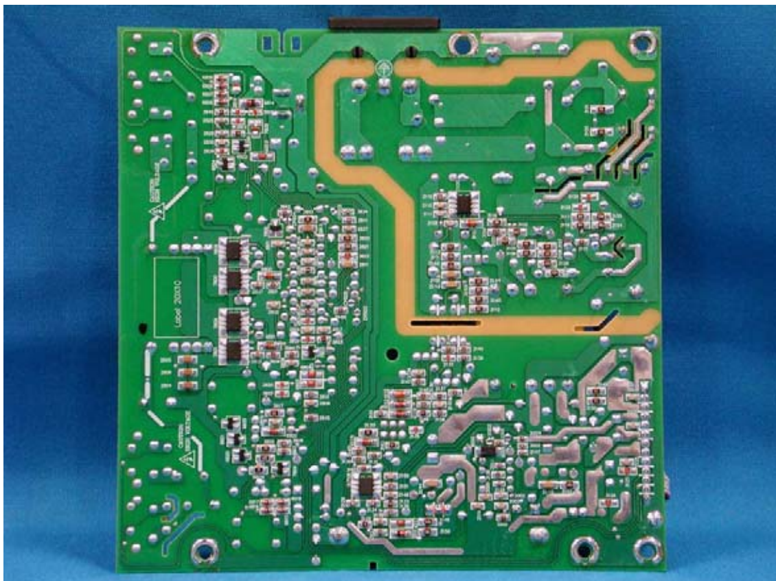
PCB Layout (Ambit T50P050.00)
