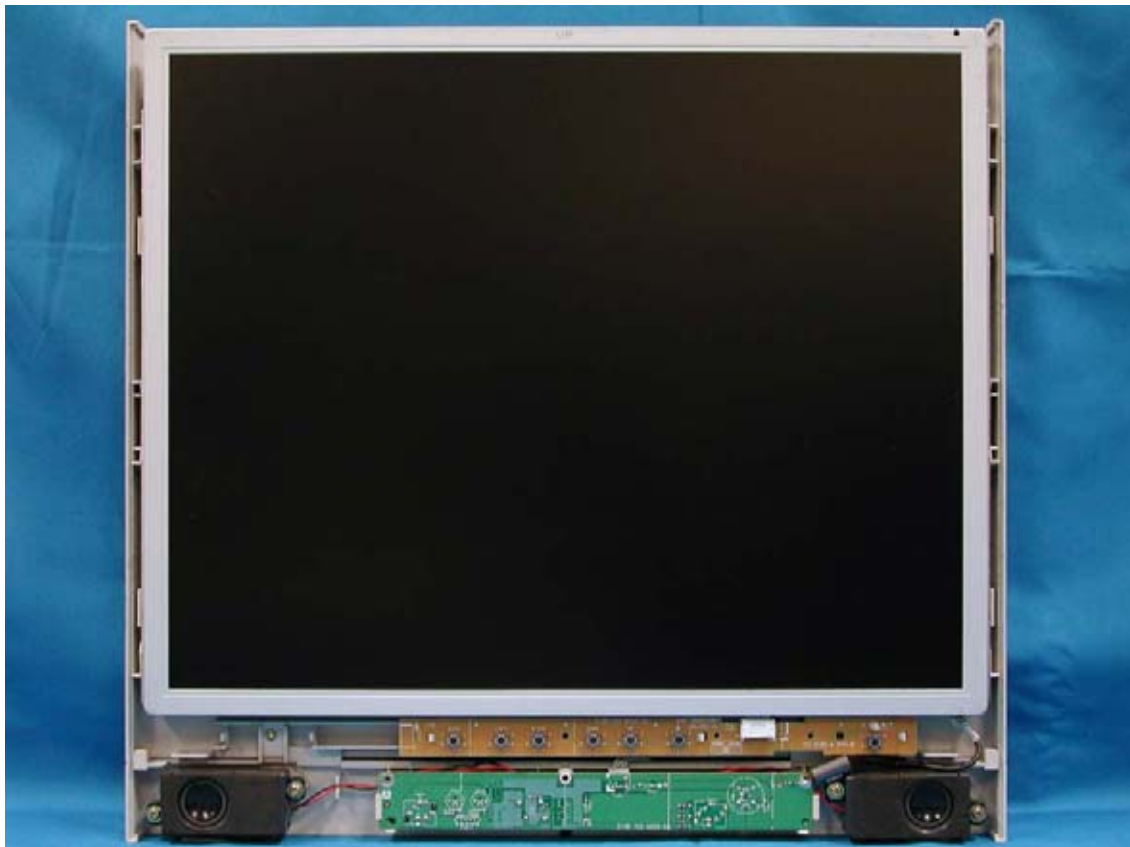
Front View w/o Front Cabinet
