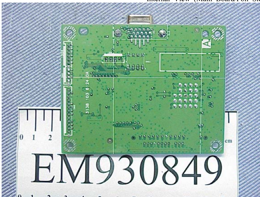
Figure 14 Internal View (Main Board/Foil Side)
