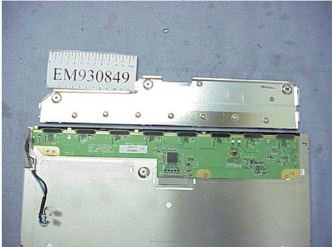
Figure 19 Internal View (Removed Metal Cover, LVDS Board)
