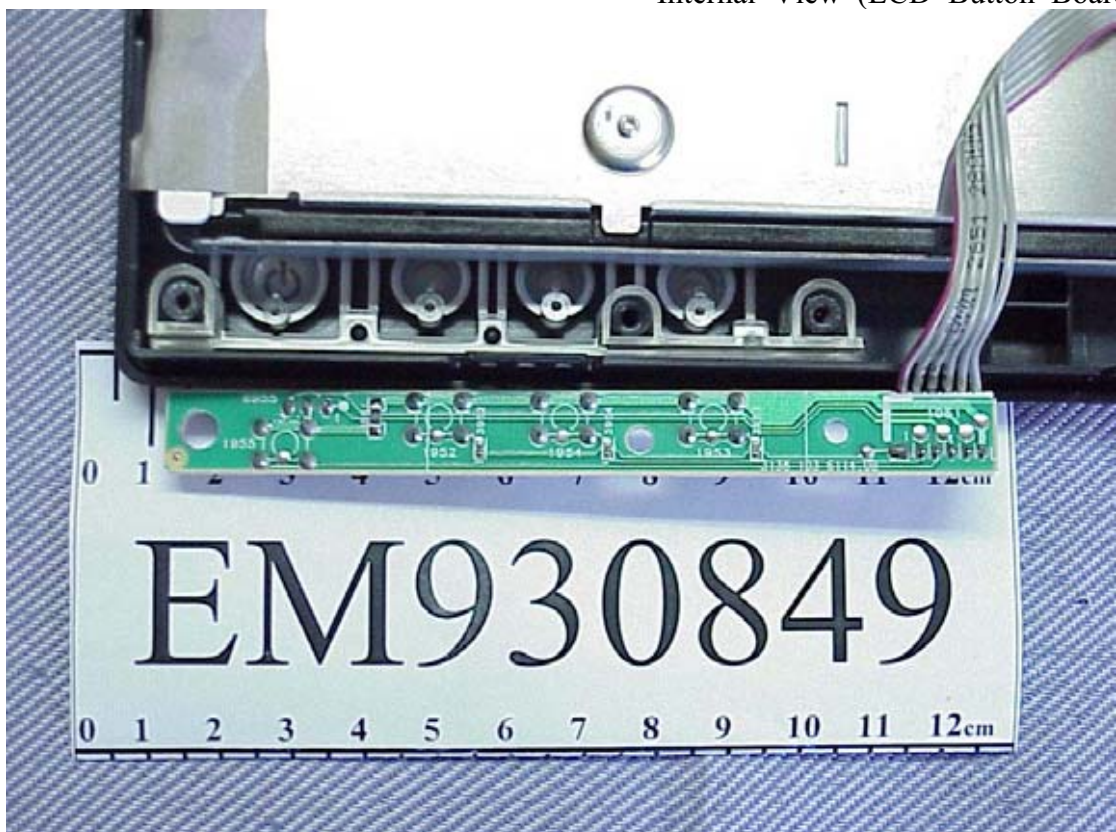
Figure 16 Internal View (LCD Button Board)
