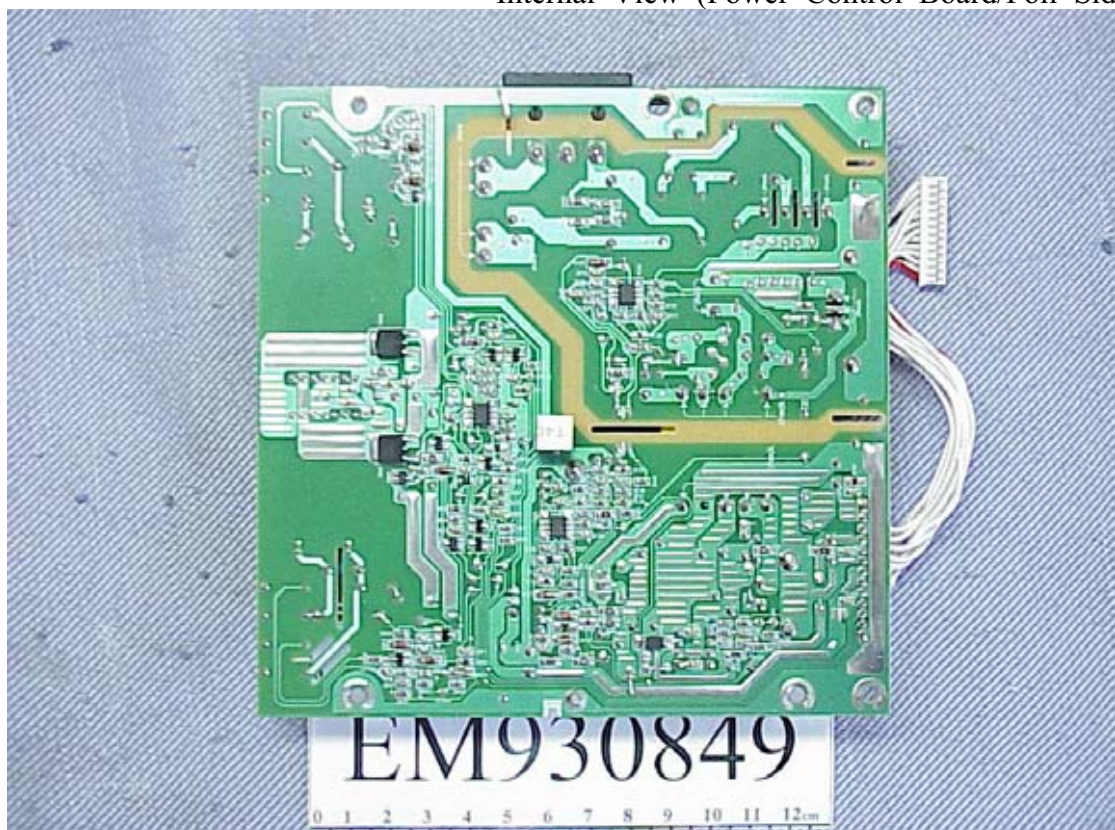
Figure 12 Internal View (Power Control Board/Foil Side)
