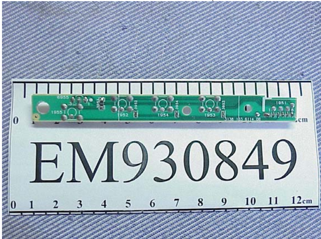
Figure 17 Internal View (LCD/Button Board/Foil Side)
