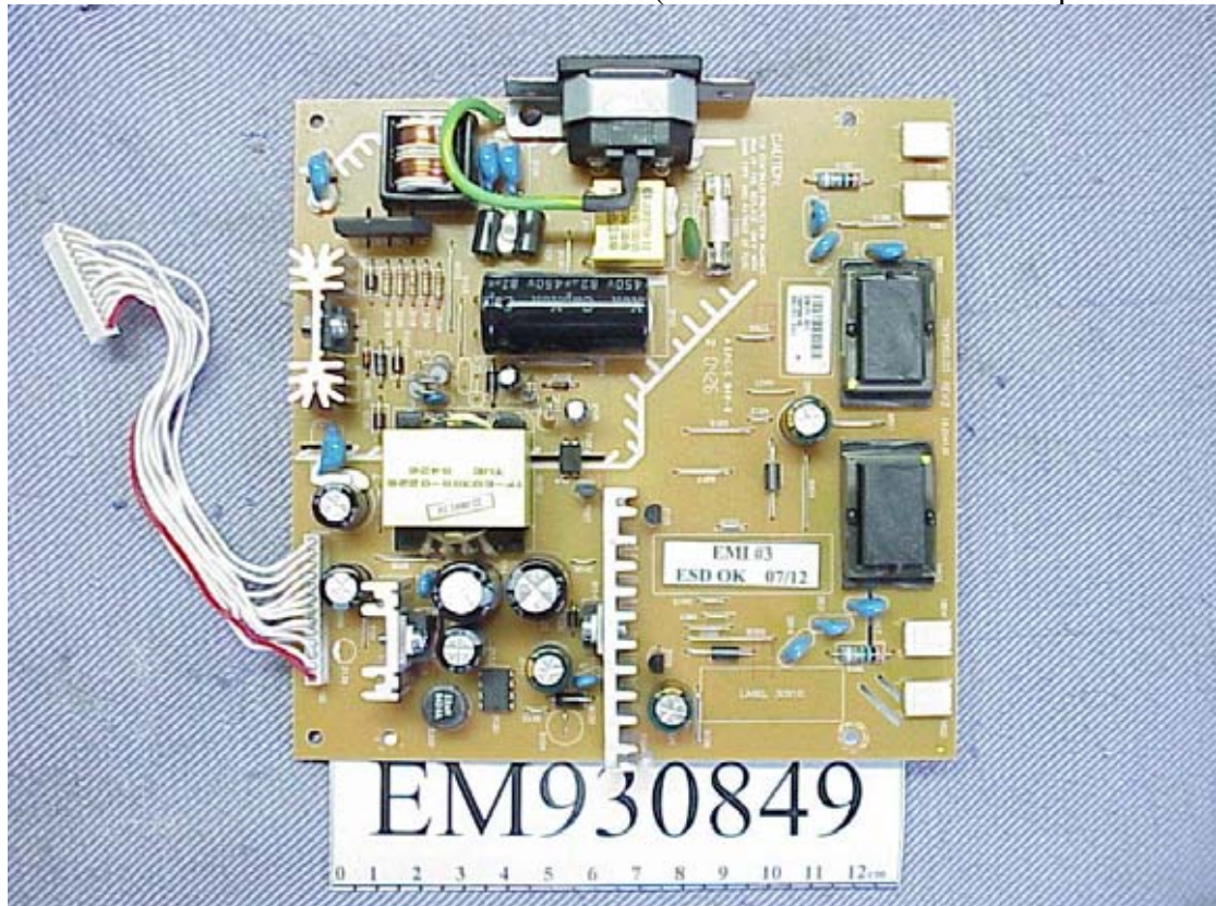
Figure 11 Internal View (Power Control Board/Component Side)
