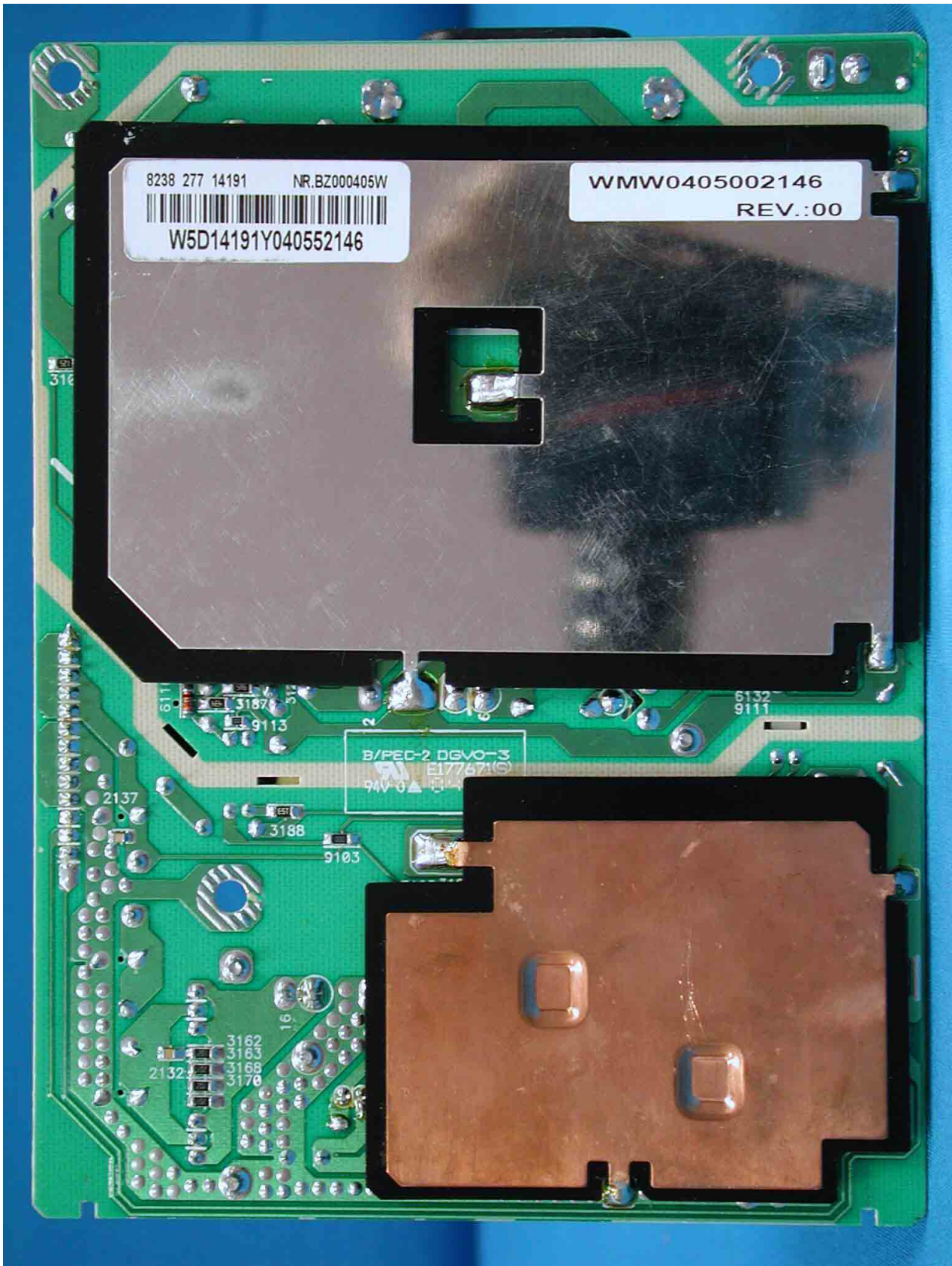
PCB Layout with shielding
