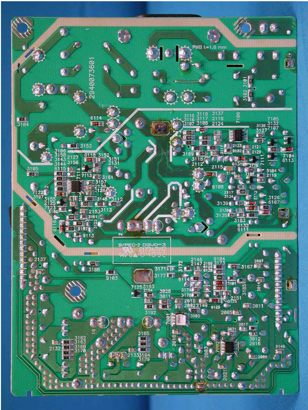
PCB Layout w/o shielding
