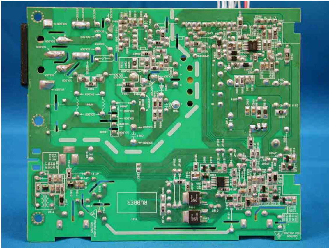
PCB Layout (LC Power)
