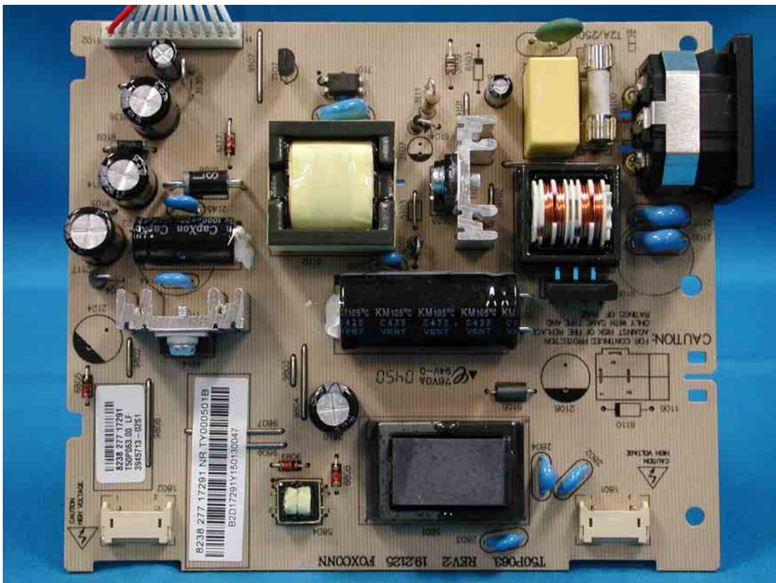
PCB Layout (Foxconn Power)
