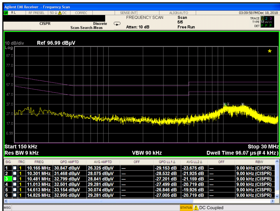
Plot 7-8. Line-Conducted Test Plot with Antenna Terminated in 50Ω (N)
