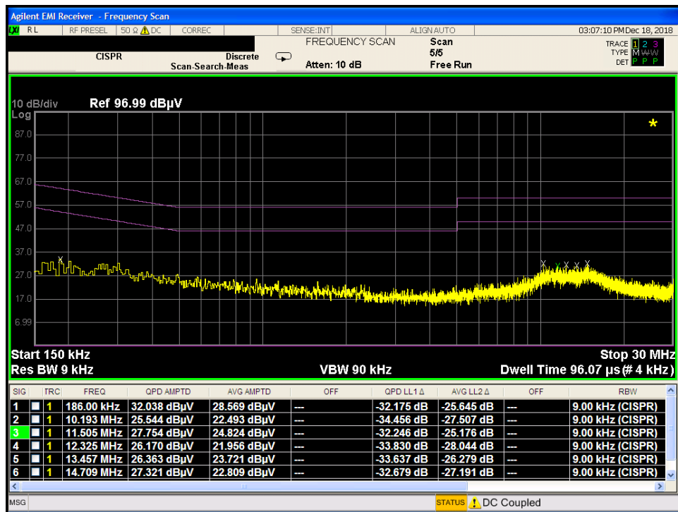
Plot 7-7. Line-Conducted Test Plot with Antenna Terminated in 50Ω (L1)
