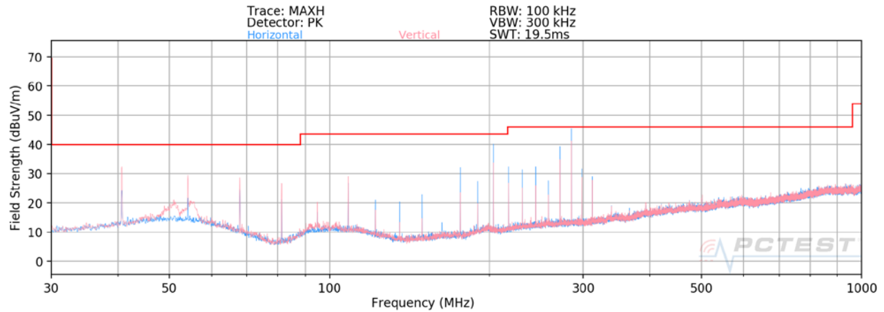
Plot 7-4. Radiated Spurious Plot 30MHz – 1GHz
