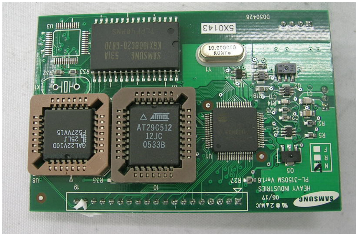
PLC Board
