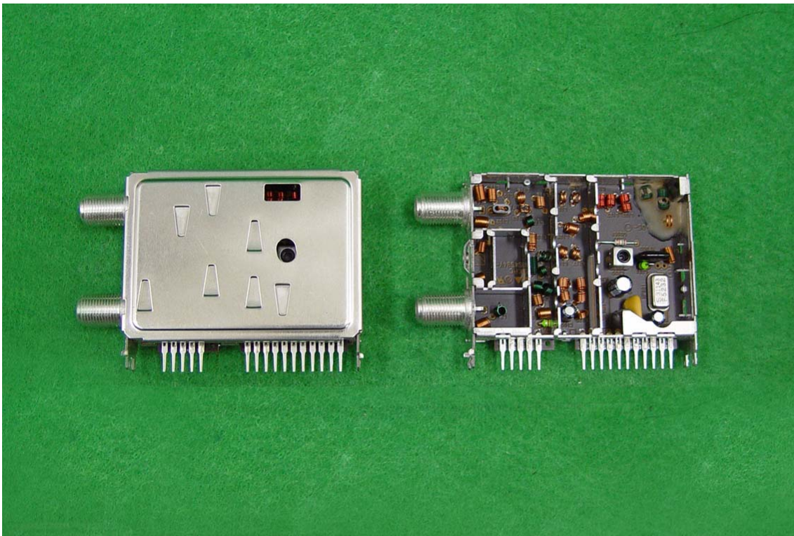
Bottom View
