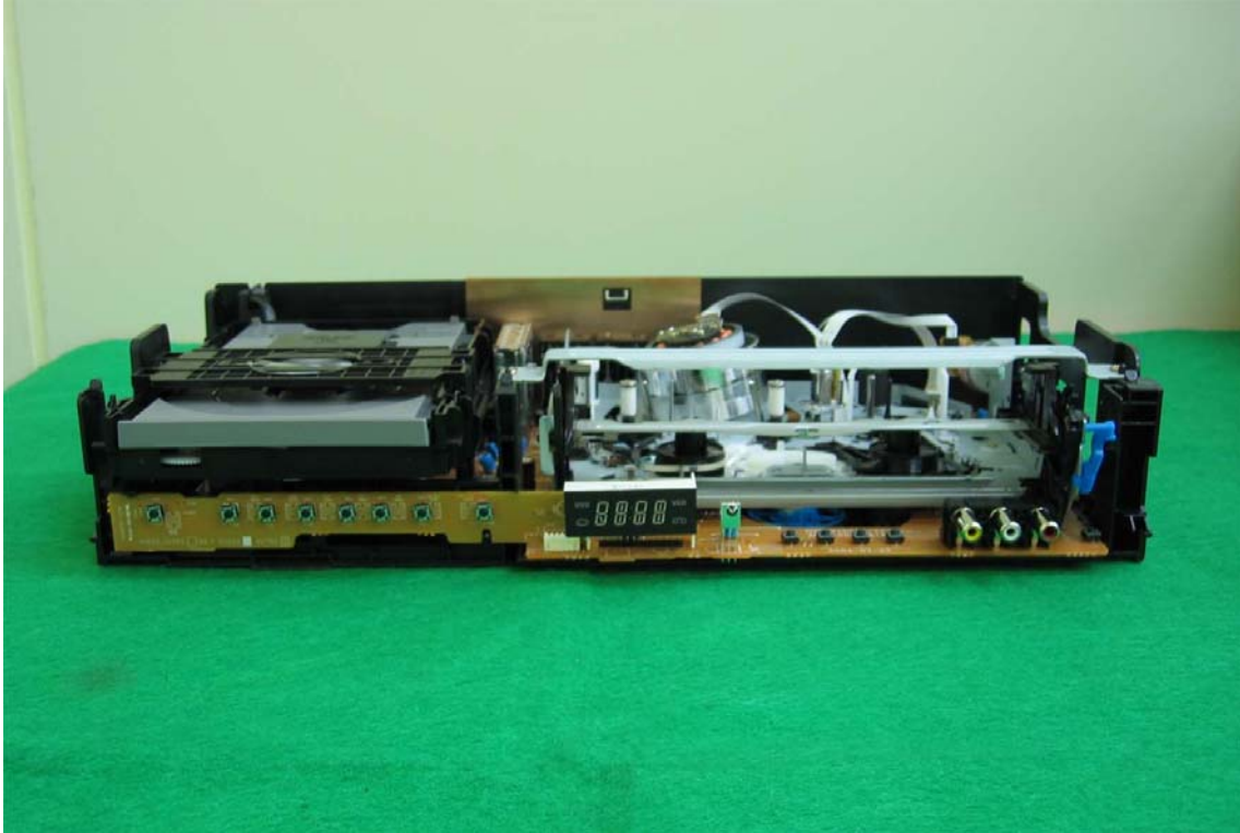
Front View – Front/Top cover open
