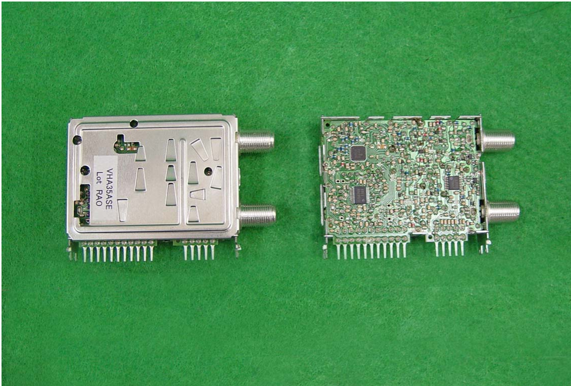
Top View
