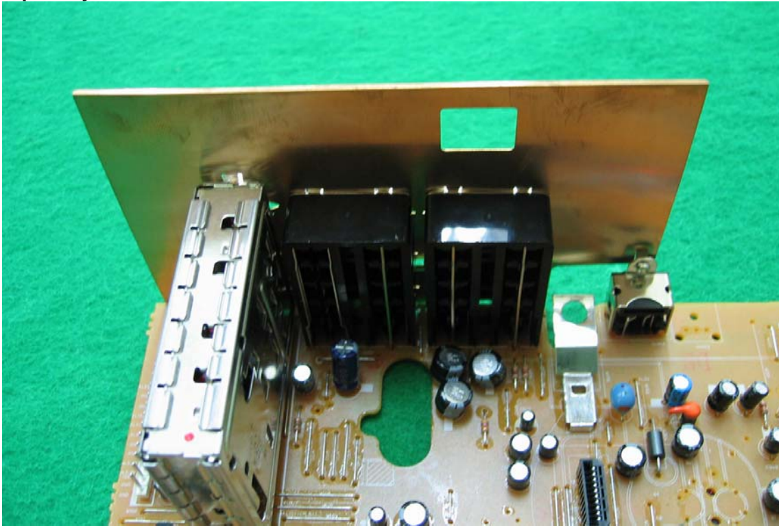
Top of Key function PCB View
