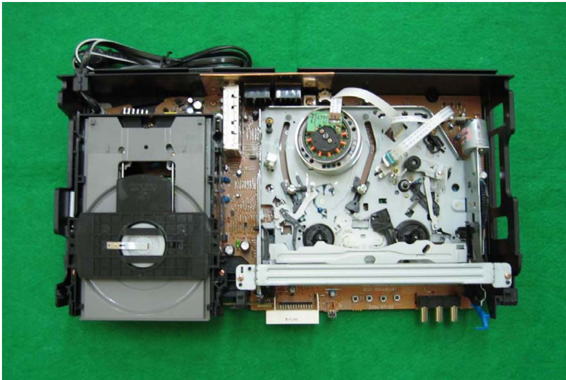
Top View – Top cover open
