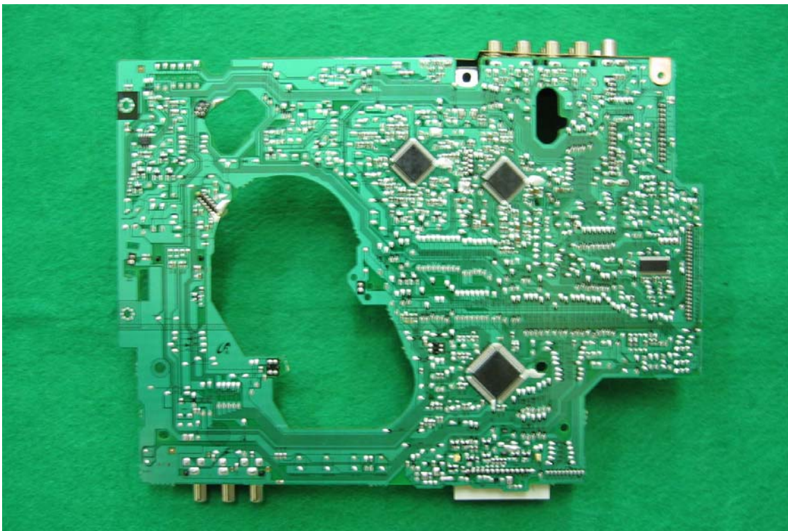
Bottom of Main PCB View
