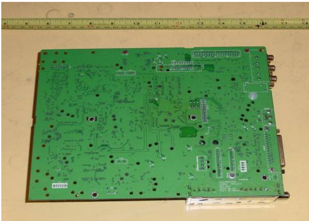
Rear of Logic Board
