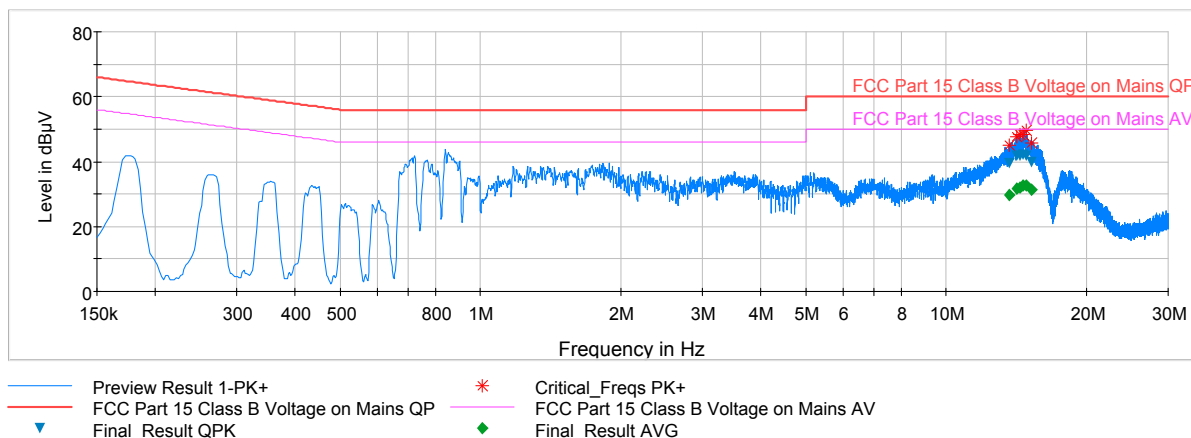
Plot 6-21. Line Conducted Plot with Bluetooth LE (N)
