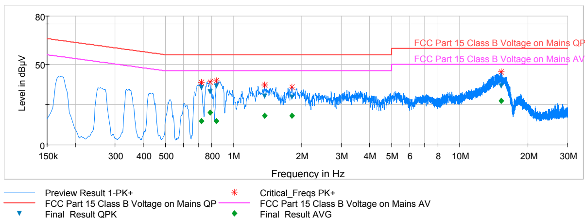
Plot 6-20. Line Conducted Plot with Bluetooth LE (L1)
