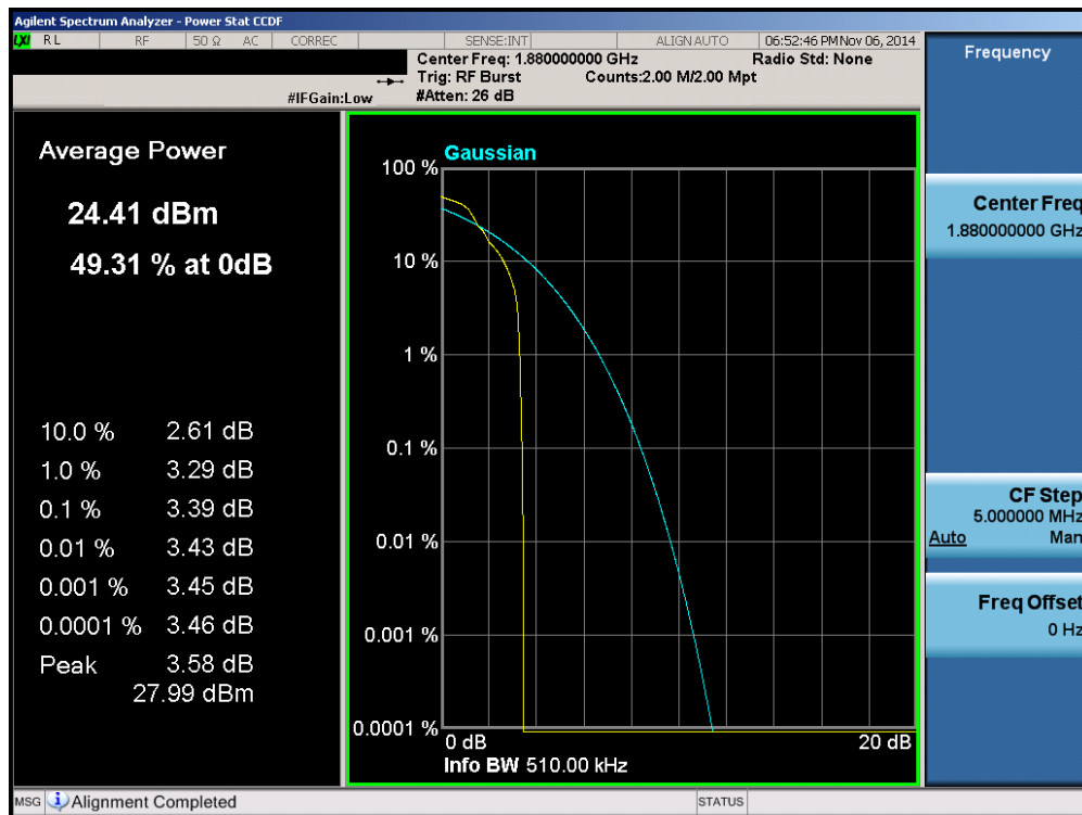
Plot 6-25. Peak-Average Ratio Plot (EDGE1900 Mode – Ch. 661)
