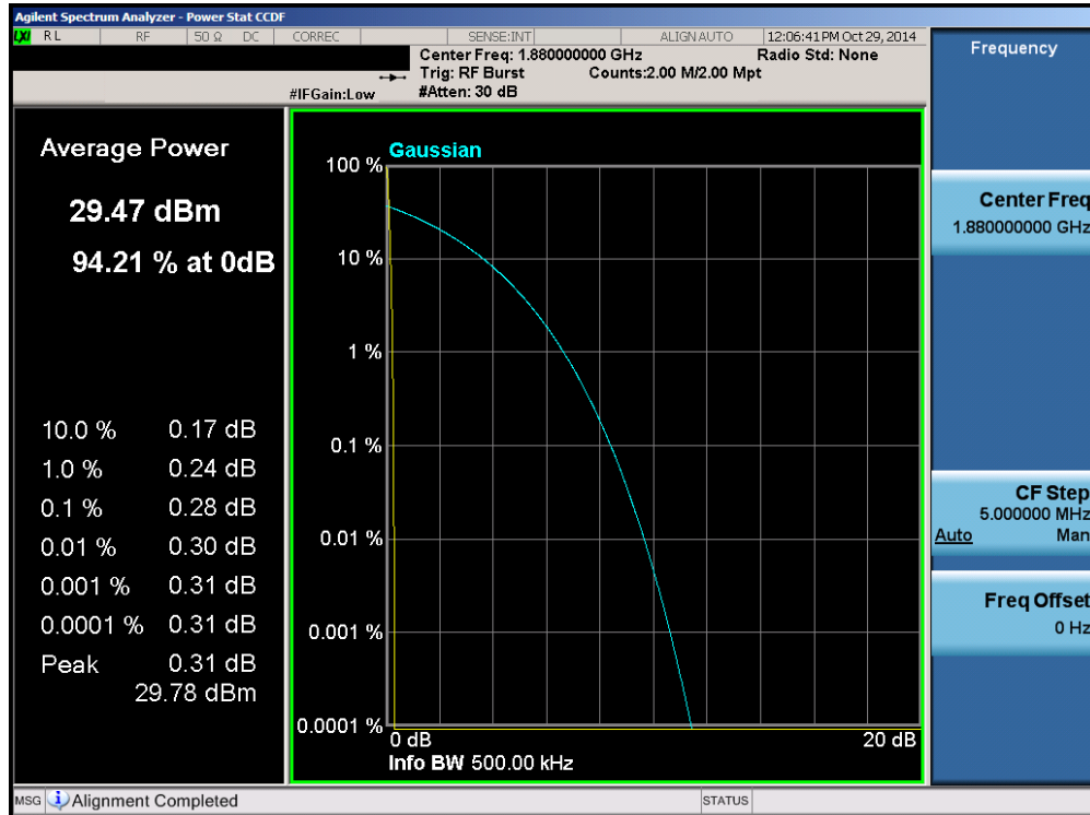
Plot 6-24. Peak-Average Ratio Plot (PCS GSM Mode – Ch. 661)
