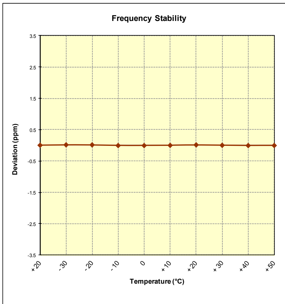
Figure 6-8. Frequency Stability Graph (PCS GSM Mode – Ch. 661)
