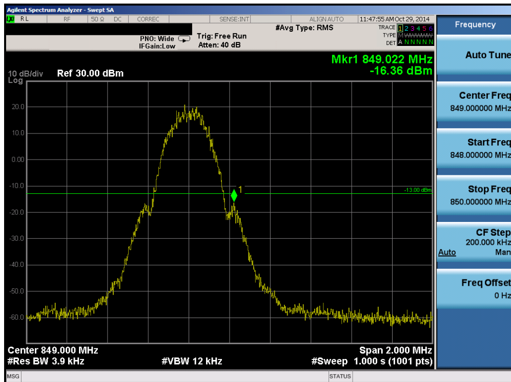
Plot 6-21. Band Edge Plot (Cellular GSM Mode – Ch. 251)
