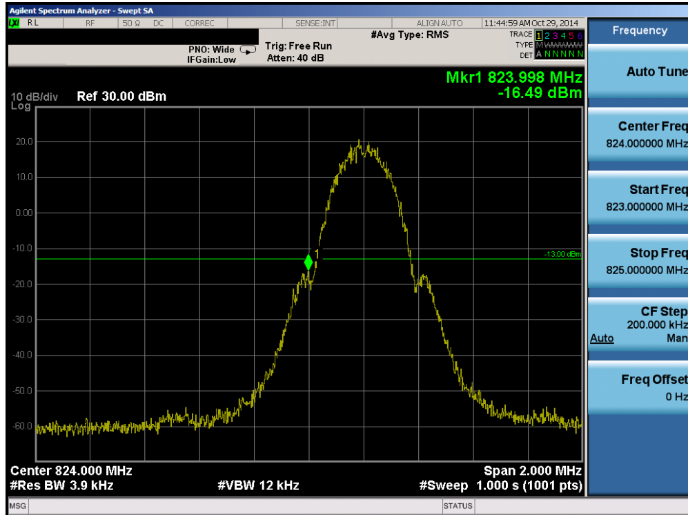
Plot 6-20. Band Edge Plot (Cellular GSM Mode – Ch. 128)
