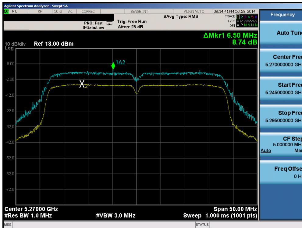
Plot 6-58. Peak Excursion Ratio Plot (40MHz BW 802.11n (UNII Band 2A) – Ch. 54)
