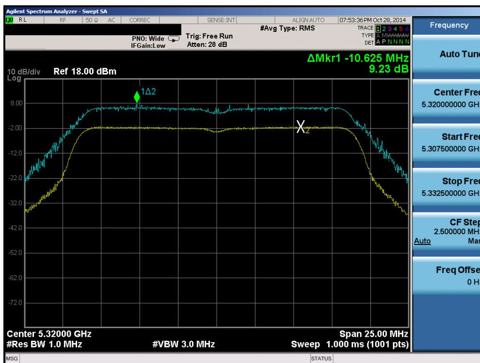
Plot 6-57. Peak Excursion Ratio Plot (20MHz BW 802.11n (UNII Band 2A) – Ch. 64)
