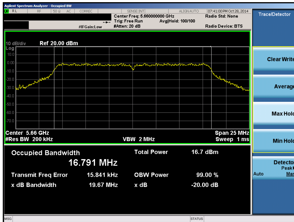
Plot 6-27. 20dB Bandwidth Plot (20MHz BW 802.11a (UNII Band 2C) – Ch. 132)
