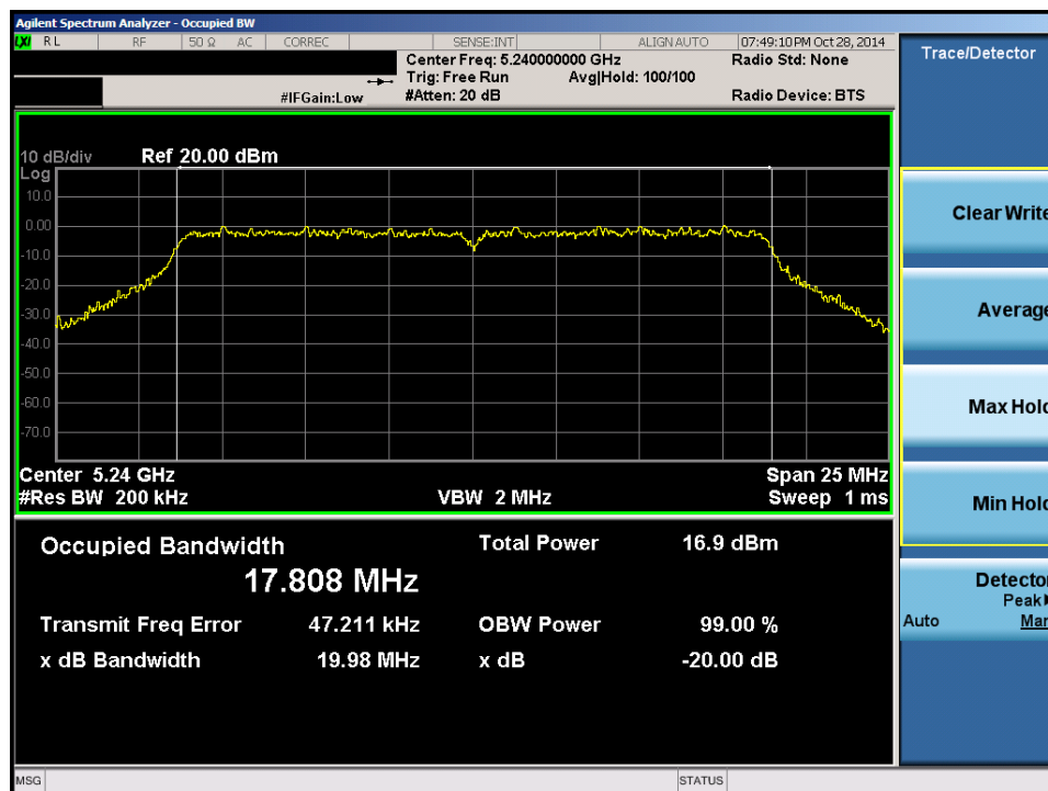
Plot 6-28. 20dB Bandwidth Plot (20MHz BW 802.11n (UNII Band 1) – Ch. 48)
