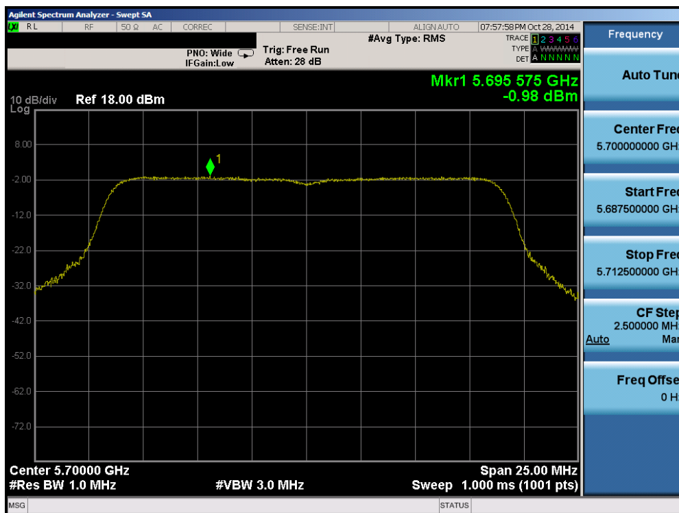
Plot 6-53. Peak Power Spectral Density Plot (20MHz BW 802.11n (UNII Band 2C) – Ch. 140)
