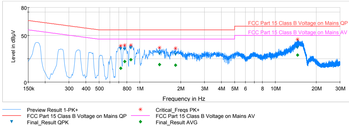
Plot 6-76. Line Conducted Plot with 802.11a UNII Band 2A (L1)
