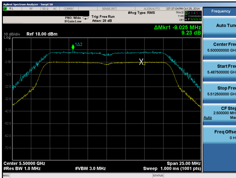
Plot 6-59. Peak Excursion Ratio Plot (802.11a (UNII Band 2C) – Ch. 100)
