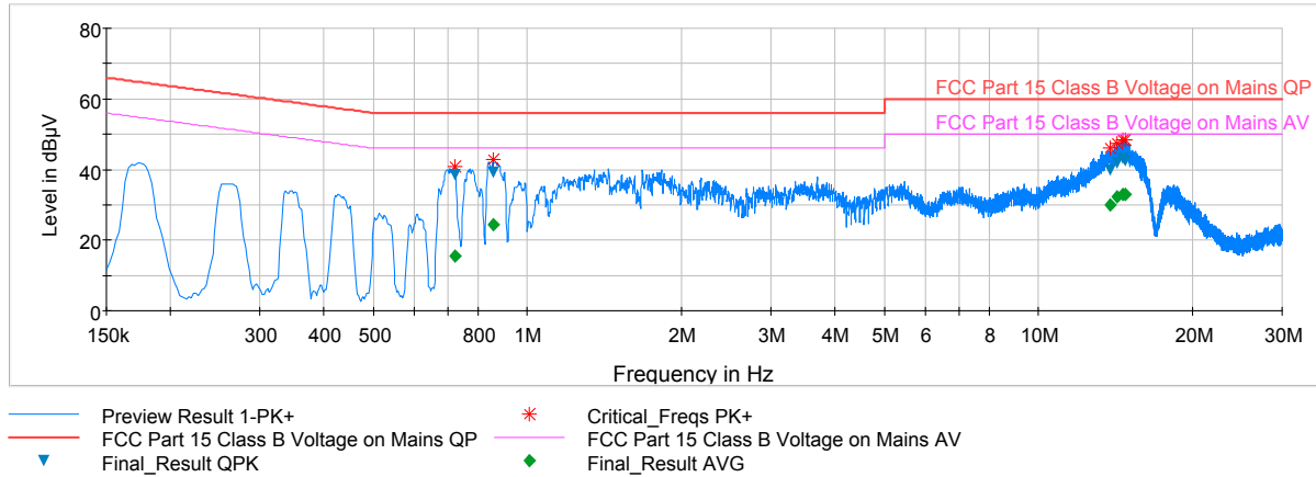
Plot 6-79. Line Conducted Plot with 802.11a UNII Band 2C (N)
