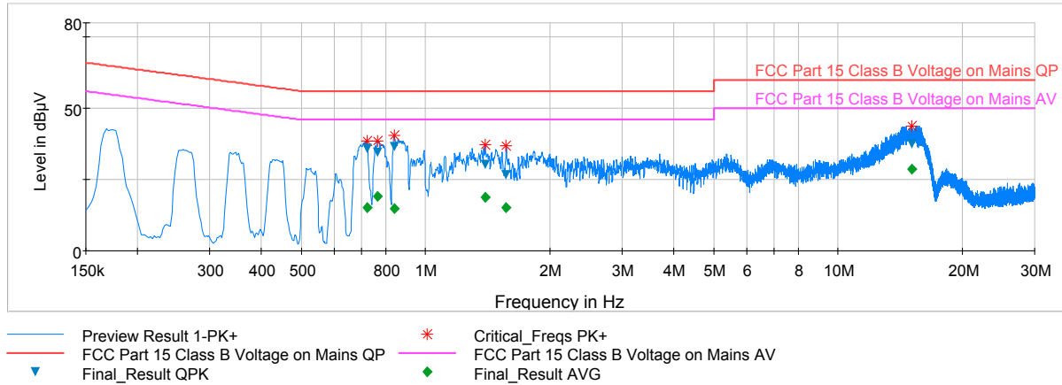
Plot 6-74. Line Conducted Plot with 802.11a UNII Band 1 (L1)
