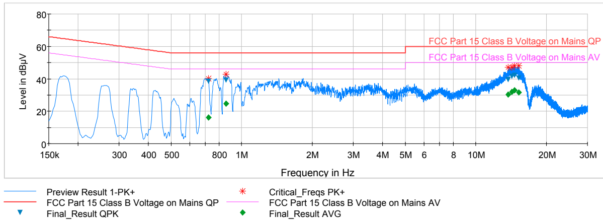
Plot 6-77. Line Conducted Plot with 802.11a UNII Band 2A (N)
