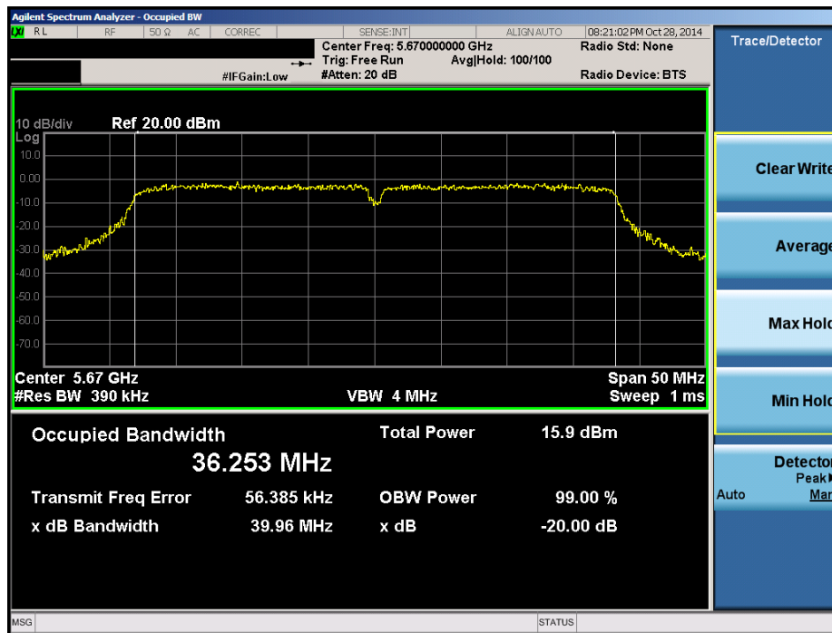
Plot 6-31. 20dB Bandwidth Plot (40MHz BW 802.11n (UNII Band 2C) – Ch. 134)
