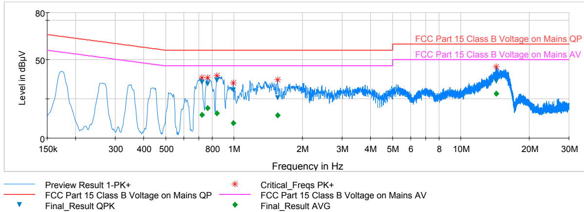
Plot 6-78. Line Conducted Plot with 802.11a UNII Band 2C (L1)
