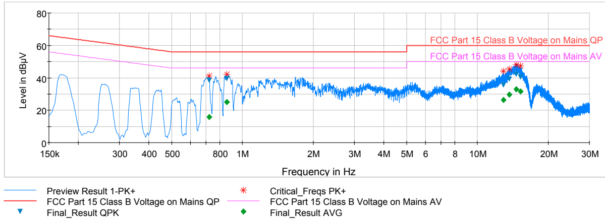
Plot 6-75. Line Conducted Plot with 802.11a UNII Band 1 (N)
