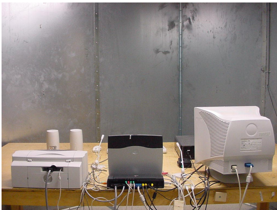
PHOTOGRAPH 6-2: CONDUCTED EMISSIONS REAR VIEW
