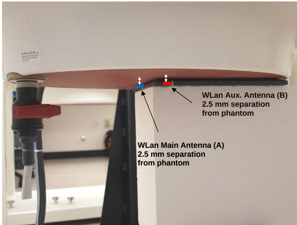
(1) Bottom face Side view
