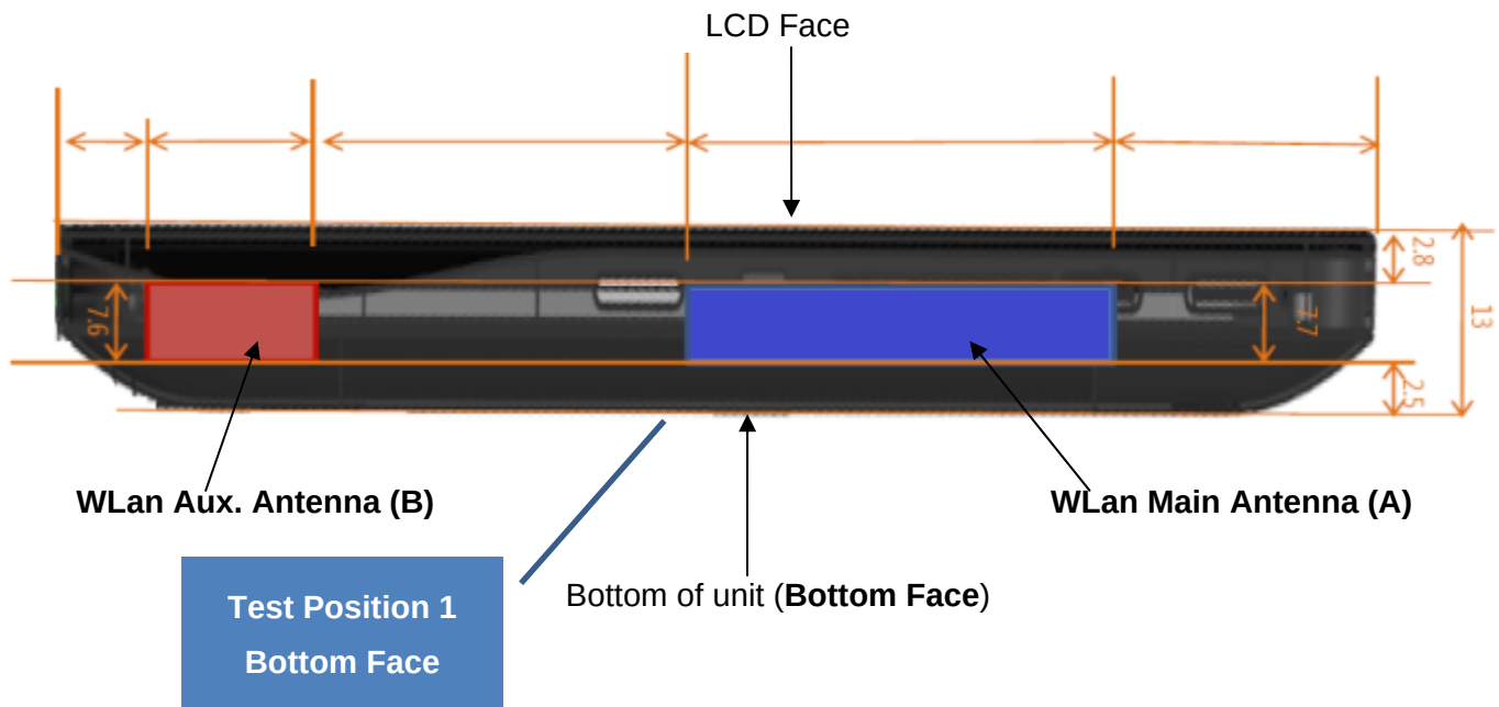
Antenna locations and separation distances
