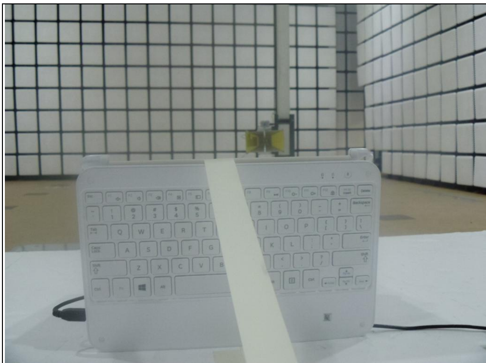
Photo of Field Strength & Spurious Emission Test(Above 1 GHz)
