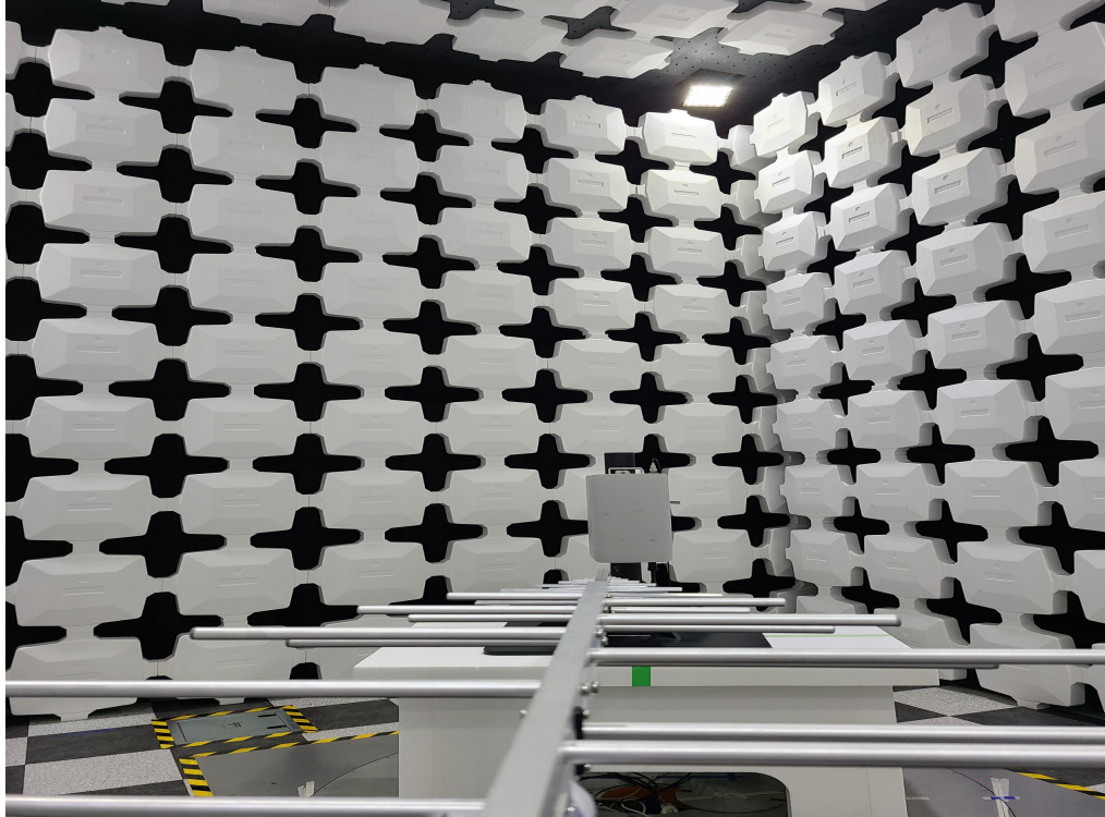
Testing setup for 18 GHz to 40 GHz
