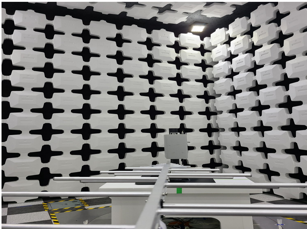
Testing setup for 30 MHz to 1 GHz
