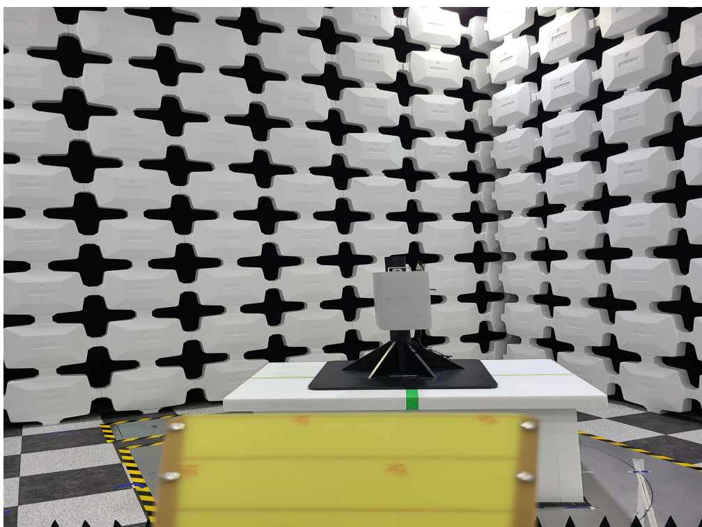
Testing setup for 1 GHz to 18 GHz
