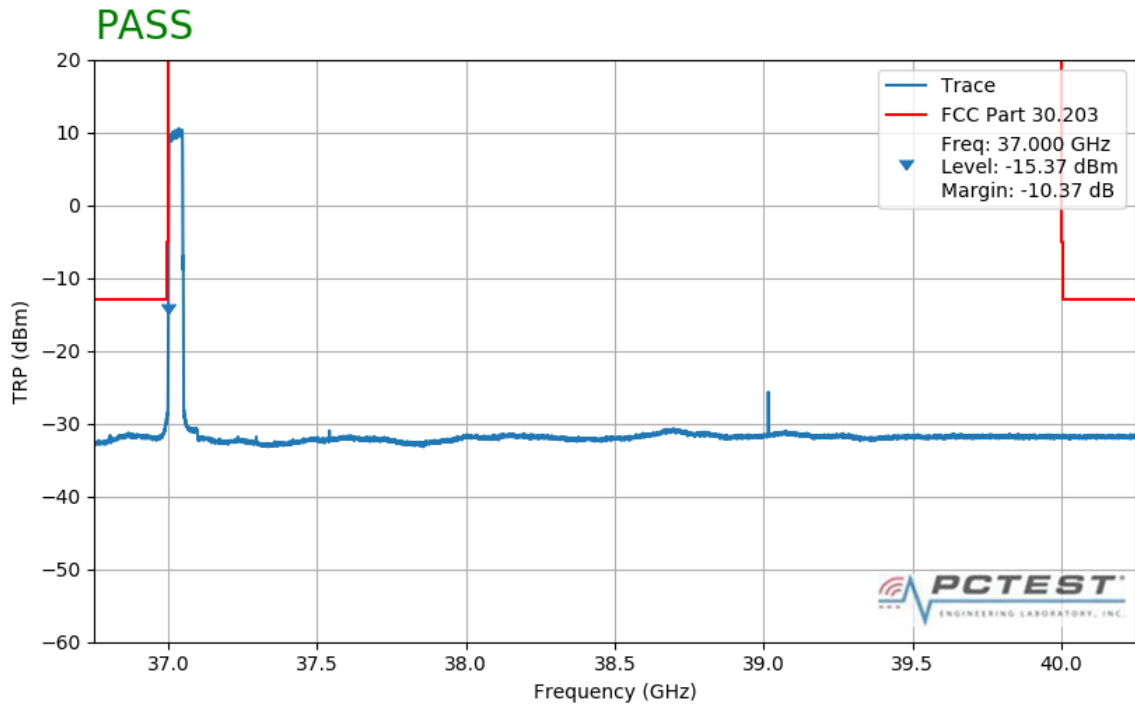
Plot 7-537. Band Edge Plot (50MHz BW 1CC QPSK Low Channel)
