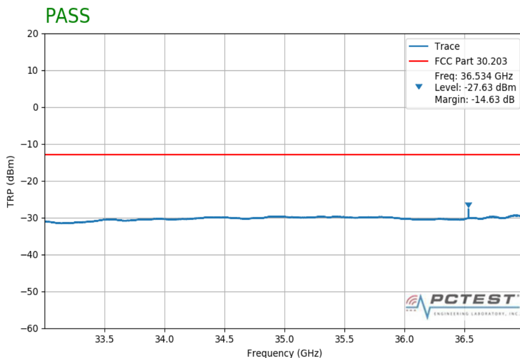
Plot 7-342. Radiated Spurious Plot 33-37 GHz (8CC NC QPSK Mid Ch. TRP)
