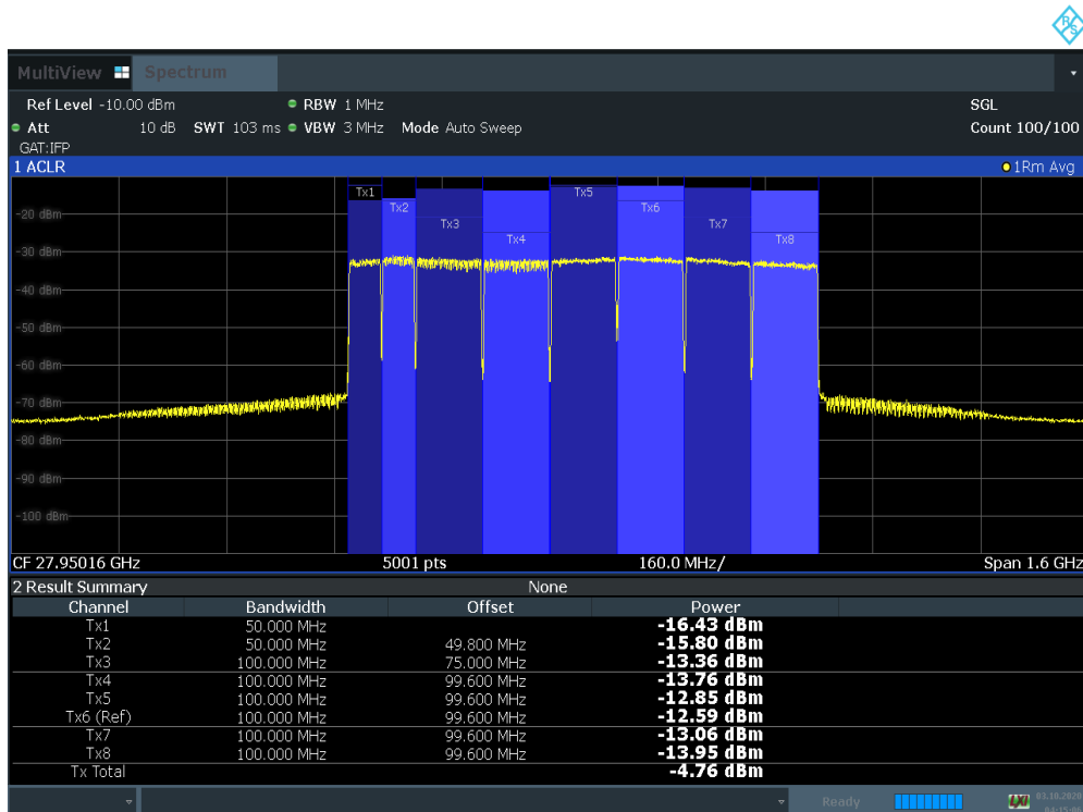
Plot 7-156. EIRP Density (Ant B 50 MHz 2CC + 100 MHz BW 6CC QPSK High)
