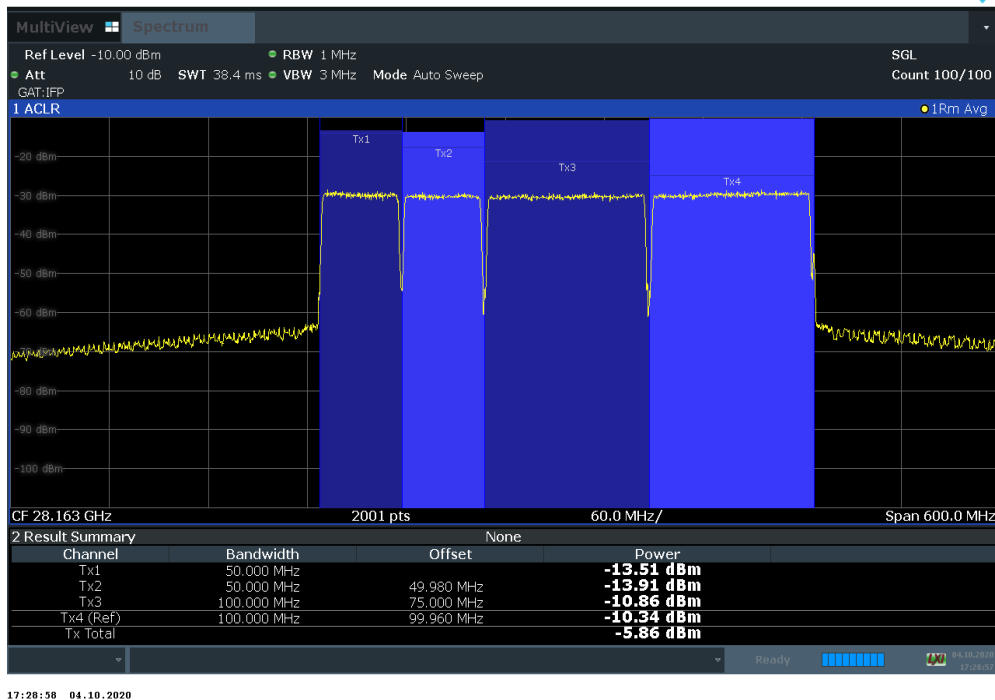
Plot 7-148. EIRP Density (Ant B 50 MHz 2CC + 100 MHz BW 2CC QPSK High)
