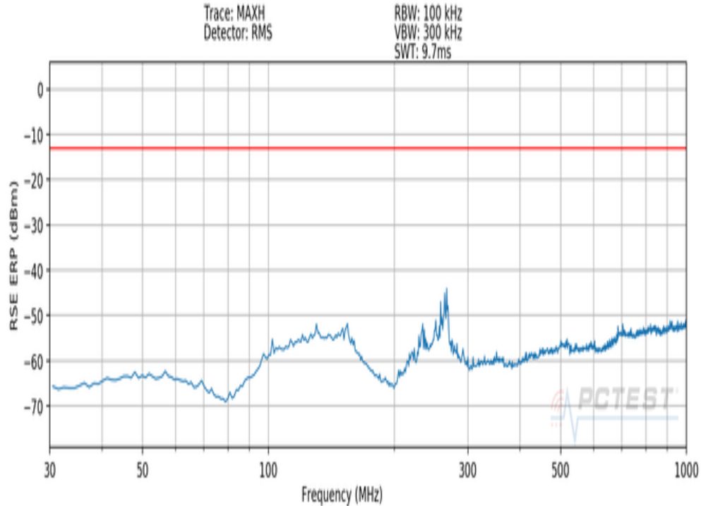
Plot 7-283. RSE 30 MHz – 1 GHz (50 MHz 2CC + 100 MHz BW 6CC CC QPSK Low Ant. Pol. H)
