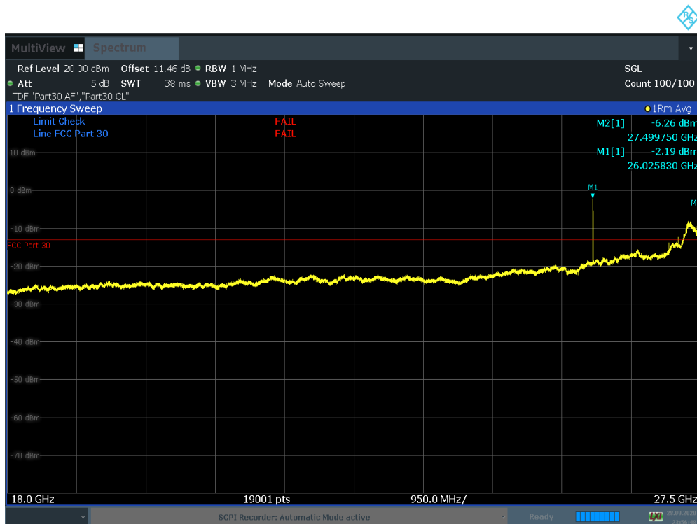
Plot 7-356. RSE 18 GHz – 27.5 GHz (100 MHz BW 4CC NC QPSK Mid Ant. Angle 135, Final)
