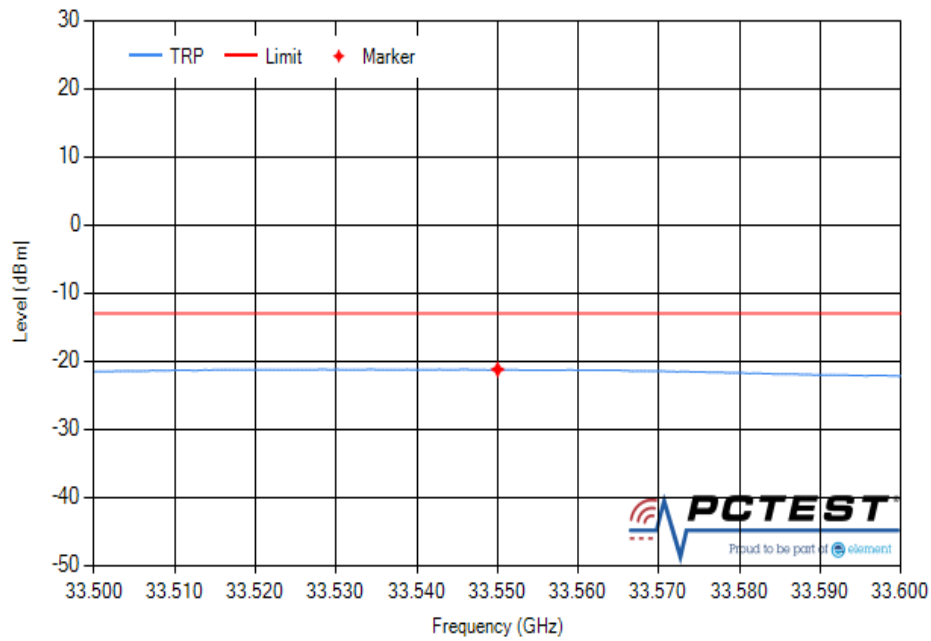
Plot 7-573. RSE 33.5 GHz – 33.6 GHz (50 MHz BW 2CC + 100 MHz BW 3CC CC QPSK Mid TRP)
