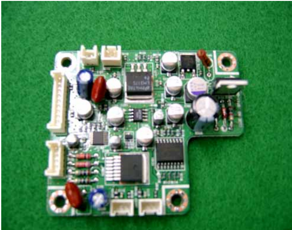
Sub detect board top view
