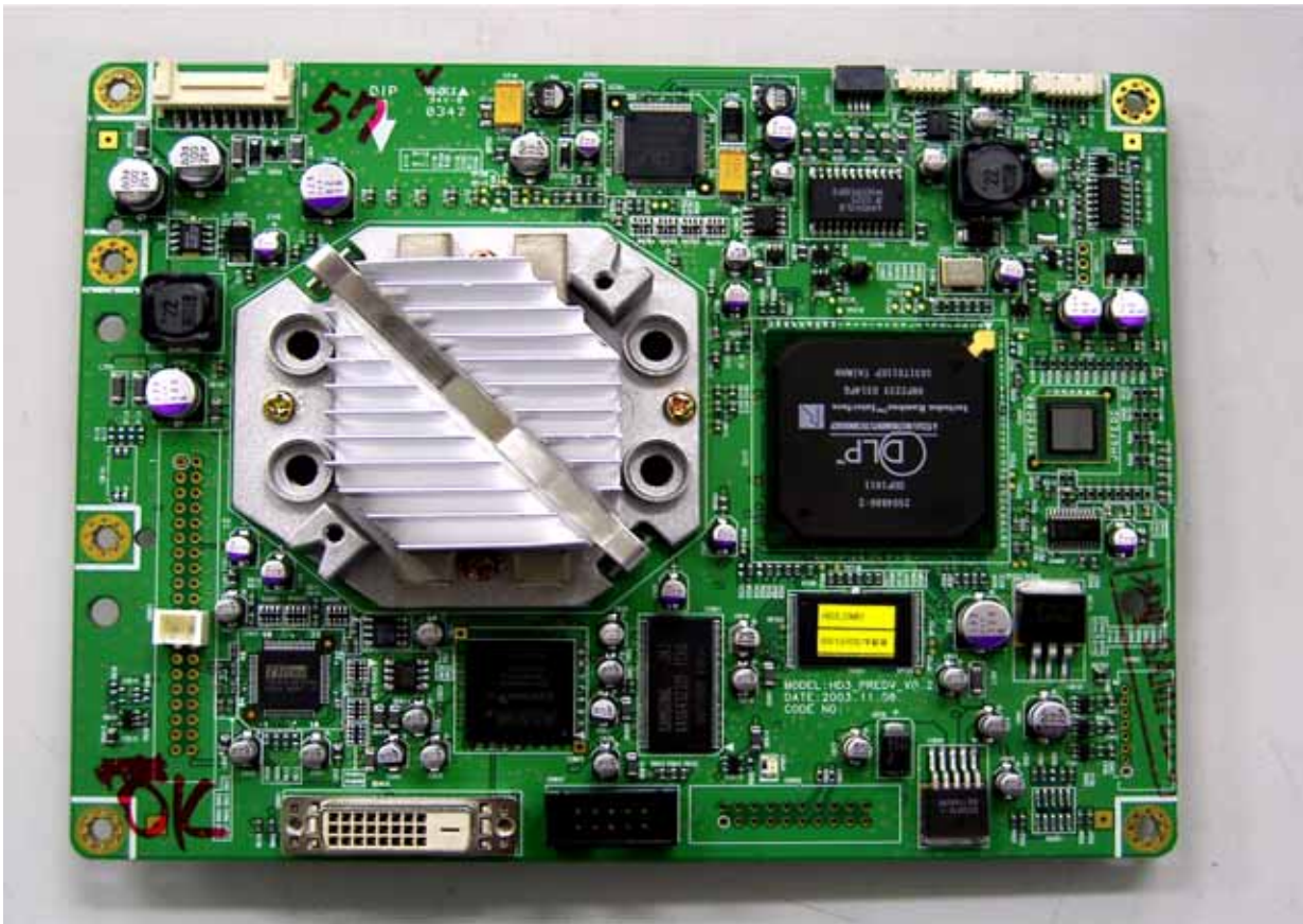
DMD board top view
