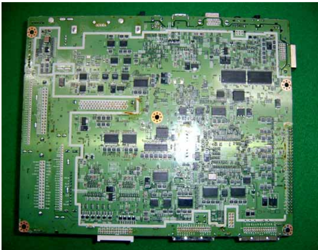
Digital board top view
