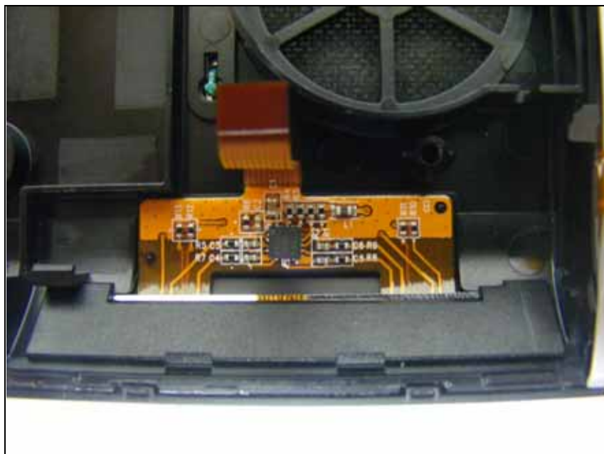
View of Sub-PCB
