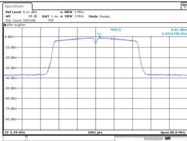
UNII-2C / 802.11ac VHT40 / High ch.
