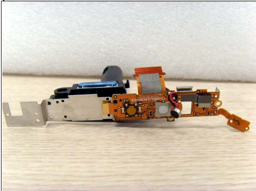
Bottom view of Flash module
