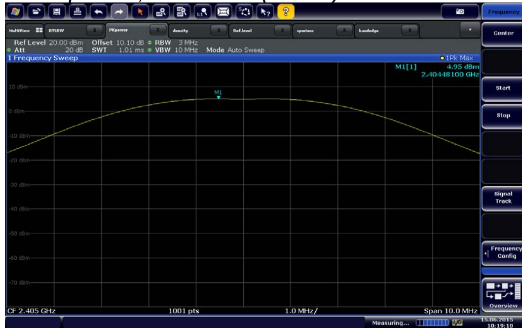
Peak Output Power, Lowest Channel (2405 MHz)
