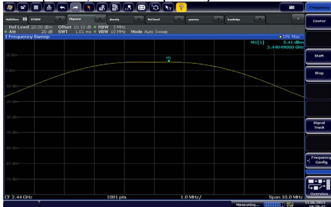
Peak Output Power, Middle Channel (2440 MHz)
