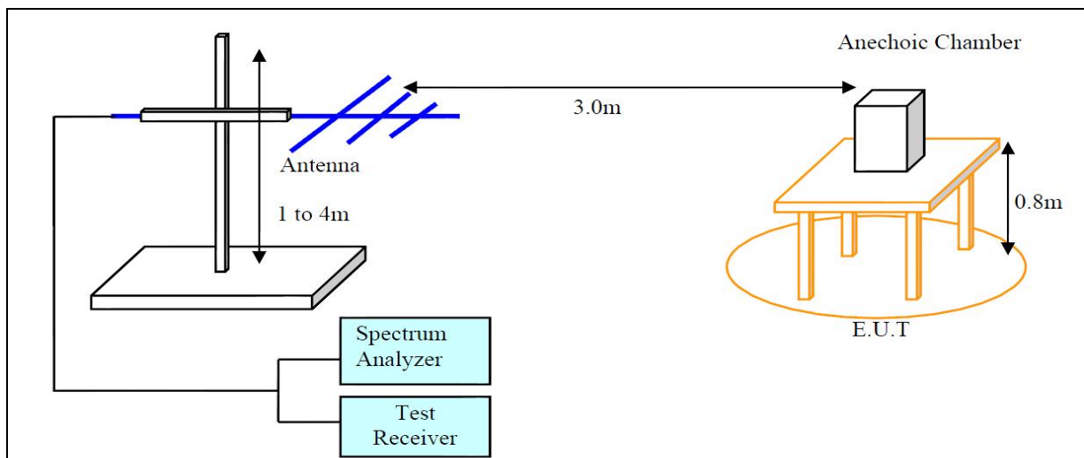
< Test setup for 30 MHz to 1GHz >
