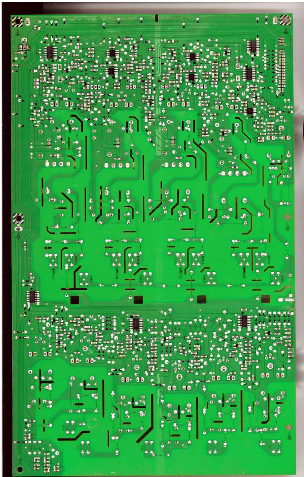
Fig. 06 HVPS Solder
