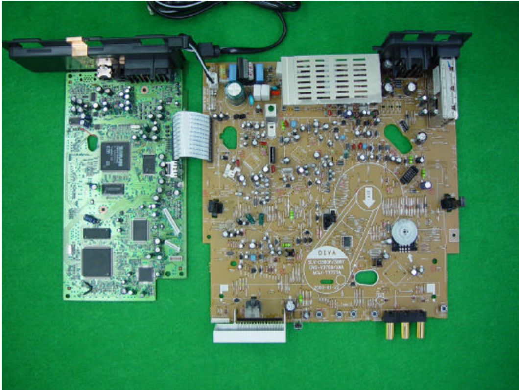
[Top of Main PCB View]
