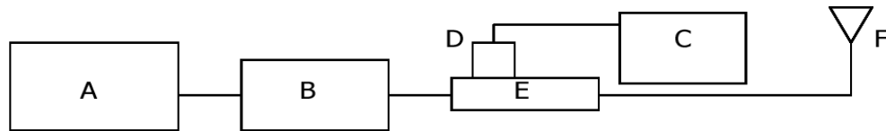
Fig 1. The microwave circuit arrangement used for SAR system verification
