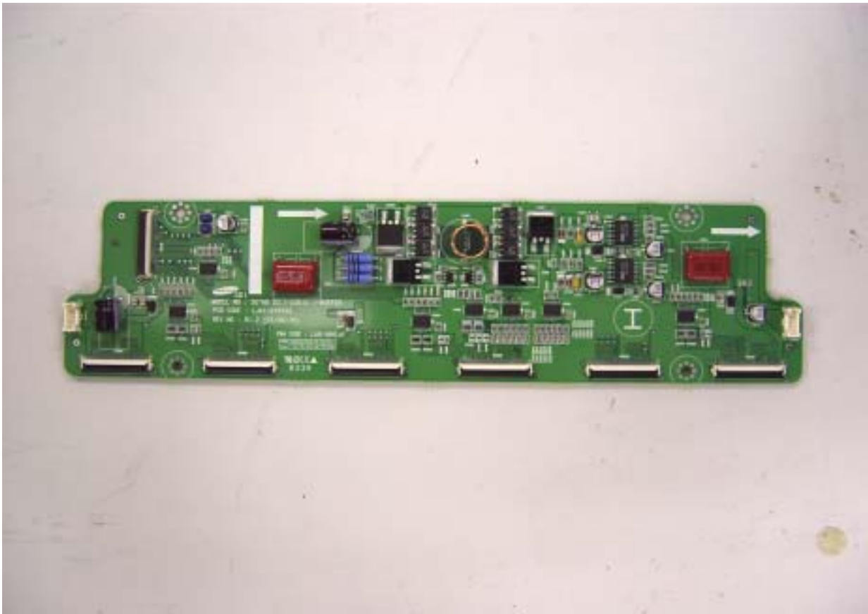
I buffer top view
