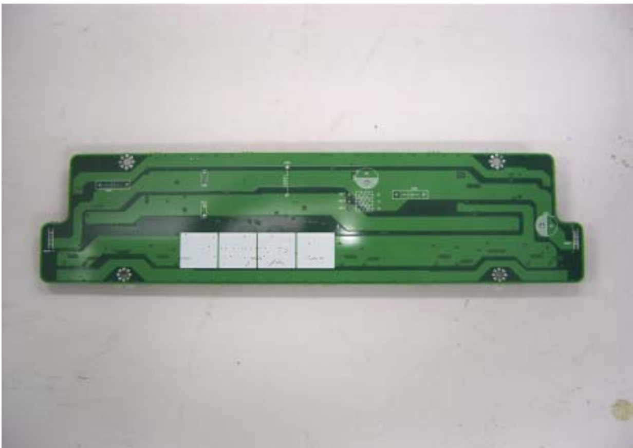
I buffer bottom view
