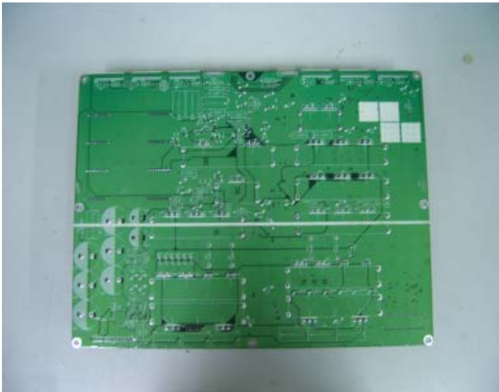
Y-Driver Board Bottom View
