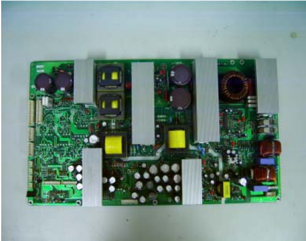
SMPS Board Top View
