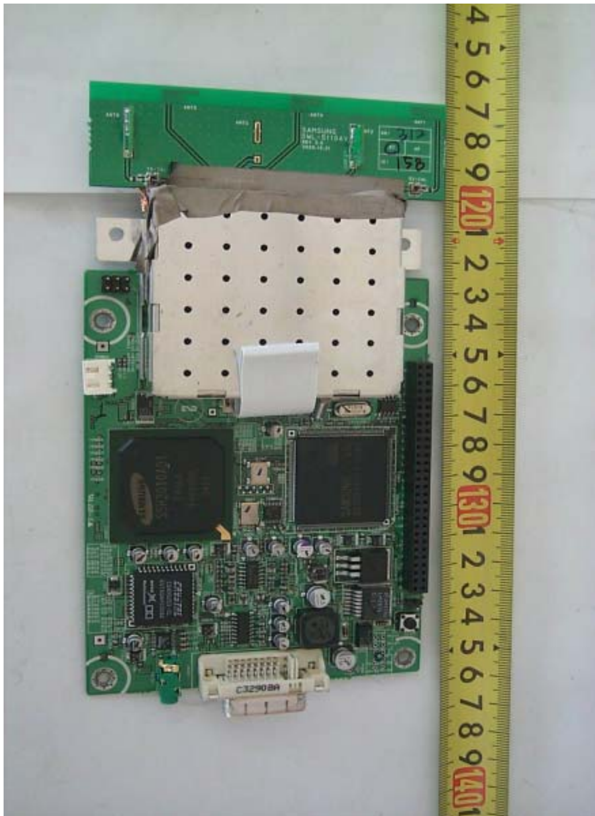
Main board Top View (Wireless Module)
