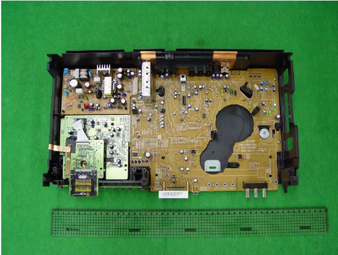
Top View – DVD/VHS Deck removed
